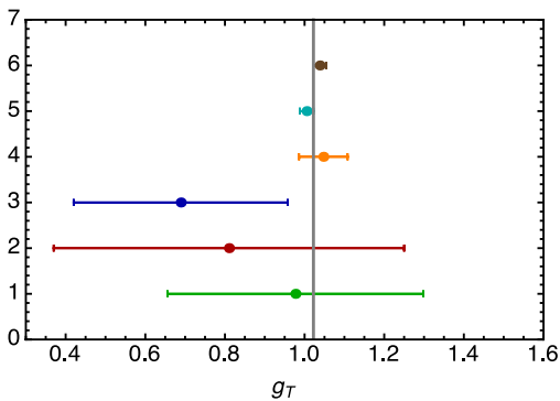
FIG. 1: (Color online) Values of the tensor charge, g_T , Eq.(5), as obtained from Lattice QCD at Q^2 = 4 \text{ GeV}^2 , and experiments, evolved to Q^2 = 4 \text{ GeV}^2 from their original scale in the range Q^2 = 1 - 3 \text{ GeV}^2 . (1) DVMP [36], (2) DiFF ( flexible form ) [35], (3) Single pion jet SIDIS [37], (4) RQCD [14], (5) LHPC [12], (6) PNDME [13]. The full line is the weighted average value of g_T .
