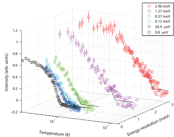
FIG. 2: (color online). Temperature dependence of the elastic channel data from \text{NiGa}_2\text{S}_4 . The nominally elastic signals of the magnetic diffuse scattering from polycrystalline \text{NiGa}_2\text{S}_4 are obtained using thermal-neutron (energy-resolution \delta E = 2.96, 1.27 meV) and cold-neutron ( \delta E = 0.37, 0.12 meV, 50.9 \mu\text{eV} ) triple-axis spectrometers at the wave vector Q = 0.58 \text{ \AA}^{-1} , and the backscattering spectrometer ( \delta E = 0.8 \mu\text{eV} ) at Q = 0.76 \text{ \AA}^{-1} [17].
