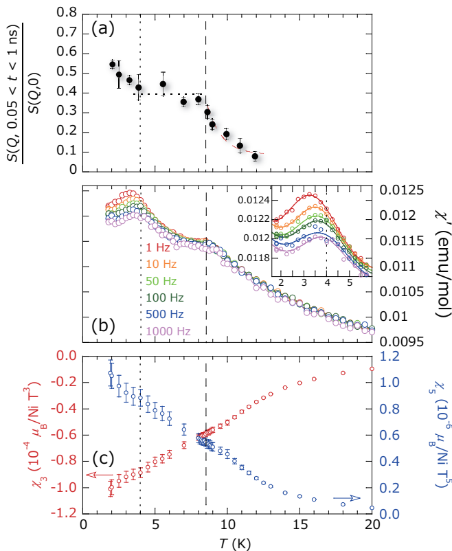
FIG. 4: (color online). Temperature dependence of (a) the averaged intermediate scattering function S(Q, 0.05 \leq t \leq 1 \text{ ns})/S(Q, 0) , (b) AC and (c) nonlinear susceptibilities, the coefficient of the third power (left-axis) and the fifth power (right-axis). The dashed curve and horizontal dotted line in (a) are guides to the eyes. The inset to (b) emphasizes the frequency dependence of \chi' at low temperatures. The vertical dashed and dotted lines denote T^* = 8.5 K and T_0 = 4 (1) K, respectively.
