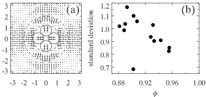
FIG. 6. (a) Mean displacement \vec{u}_{\text{avg}}(x, y) of droplets near a T1 event – four circles are the mean positions of droplets undergoing a T1 event and the axes are in units of \langle d \rangle . The mean displacement field does not vary with \phi , so data are averaged from all experiments, and four-fold symmetry is imposed. (b) We compute the standard deviation at each (x, y) between the mean flow field \vec{u}_{\text{avg}}(x, y) and the flow fields \vec{u}_i(x, y) around each T1 event i . The standard deviation is spatially averaged within a ring of radius 1.2\langle D \rangle \leq R \leq 2.0\langle D \rangle around the T1 event centers (dashed circles in (a)), and is plotted in (b) as a function of area fraction. \vec{u}_i(x, y) is normalized by the mean displacement of the T1 droplets for each \phi , so a value of 1 in the standard deviation means that the variability of droplet displacements is equal to the magnitude of the displacement of the T1 droplets.
