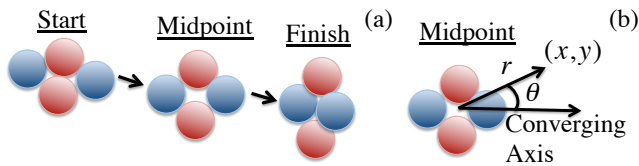
FIG. 2. (Color online). (a) T1 event, where 4 droplets exchange neighbors. (b) Coordinate system relative to midpoint of T1 event. The converging axis is the line joining the centers of the two droplets moving closer together; the direction of the axis is arbitrary. This axis defines the Cartesian coordinates (x, y) and polar coordinates (r, \theta) .
