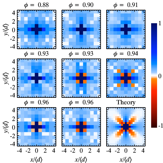
FIG. 4. (Color online). Measured stress propagators. The last panel is the theoretical stress propagator for \phi = 1 [13]. Blue indicates an average stress decrease and red indicates a stress increase. Distance to center of T1 event is measured in units of average droplet diameters. Both \phi = 0.93 panels and both \phi = 0.96 panels are two different samples with the same \phi , indicating that the stress propagator is not completely reproducible between experiments. To improve statistics in each panel, we impose four fold symmetry on \Pi . Prior to imposing symmetry, the raw data have four fold symmetry within the statistical noise limit.
