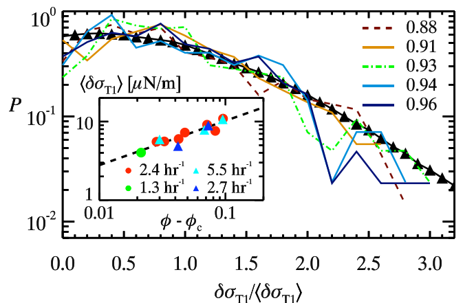
FIG. 3. (Color online). Distribution of stress decrease on the rearranging droplets. The color of the curve indicates area fraction. The solid curves are data at \dot{\gamma} = 5.5 \text{ hr}^{-1} , the dashed lines at \dot{\gamma} = 2.7 \text{ hr}^{-1} , and the dashed dot lines at \dot{\gamma} = 2.4 \text{ hr}^{-1} . The filled triangle black curve is the distribution of individual droplet shear stresses \sigma_i in a sample at \phi = 0.89 , normalized by \langle \sigma_i \rangle . Inset: Average stress relaxation with area fraction. The legend indicates data at different strain rates. The black dashed line is a power law fit \langle \delta \sigma \rangle = A(\phi - \phi_c)^\beta , where \beta = 0.57 , A = 38 \text{ } \mu\text{N/m} , and \phi_c = 0.86 .
