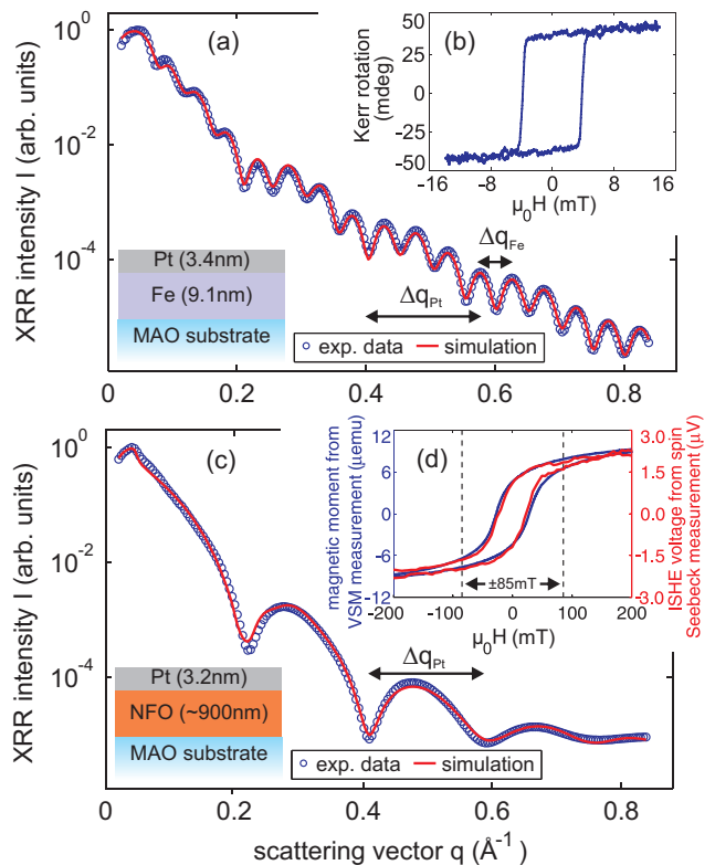
FIG. 1. (a) XRR intensity I and simulation for Pt/Fe/MAO. (b) MOKE data ( \lambda = 488 \text{ nm} ) for Pt/Fe/MAO. (c) XRR intensity I and simulation for Pt/NFO/MAO. (d) VSM and LSSE measurements ( \Delta T = 18 \text{ K} ) for Pt/NFO/MAO.
