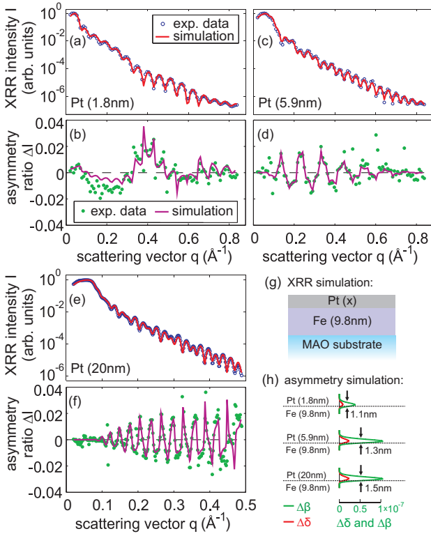
FIG. 4. XRR intensity I and corresponding asymmetry ratios \Delta I for Pt( x )/Fe(9.8 nm) with (a),(b) x = 1.8 nm (average of 8 curves), (c),(d) x = 5.9 nm and (e),(f) x = 20 nm. For the XRR simulations the model in (g) and for the asymmetry simulations the magneto-optic profiles in (h) are used.
