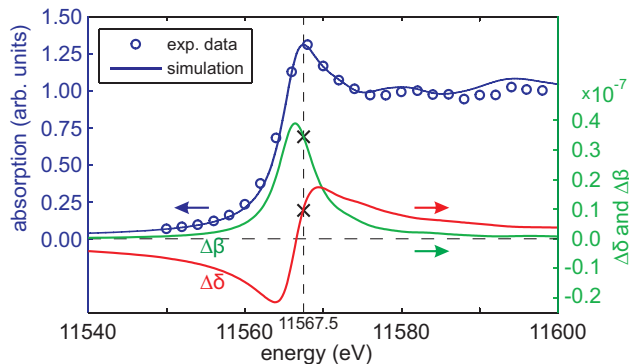
FIG. 2. Fluorescence spectrum at the Pt L_3 edge of Pt(3.4 nm)/Fe(9.1 nm) sample and simulation, both normalized to the edge jump. \Delta\delta and \Delta\beta are derived from the simulation of the absorption resulting from a magnetic moment of 0.2 \mu_B per Pt atom. XRMR was performed at the absorption maximum of 11567.5 eV (dashed vertical line) yielding a ratio \Delta\beta/\Delta\delta of 3.4 (black crosses).
