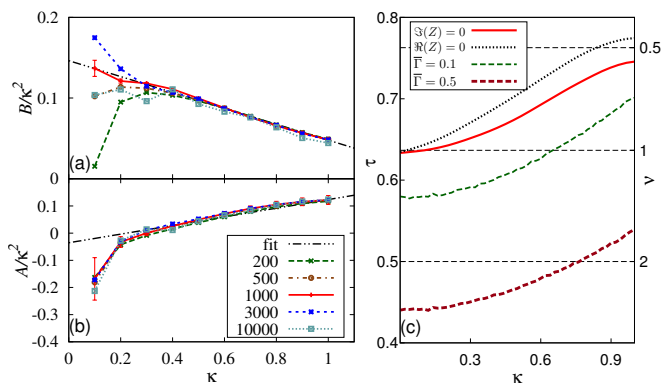
FIG. 2: (Color online) Scaled fit coefficients: (a) B/\kappa^2 and (b) A/\kappa^2 with A and B defined in Eq. (8) are plotted as functions of \kappa for GOE ensembles of different dimension N as indicated in the figure. For N = 1000 the error in the fit is shown by error bars. The errors for the other curves are similar. The double-dot-dash black line shows the linear fits (9) of A/\kappa^2 and B/\kappa^2 as functions of \kappa . Right: (c) The coefficient \tau defined in Eq. (10) is plotted versus \kappa for different widths of multiple random gamma channels as explained in the text. The scale on the right shows the corresponding \nu values.
