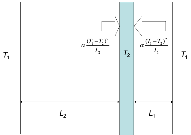
FIG. 1: Schematic illustration of Casimir pressures p_{\text{NE}}^w > 0 , induced by NE concentration fluctuations on a plate with temperature T_2 located in a liquid mixture between walls with temperature T_1 . For p_{\text{NE}}^w < 0 , the plate would be pulled to the closest wall.
