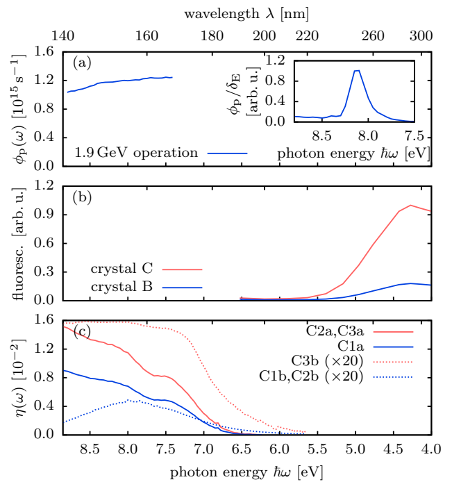
Figure 2: Photon energy (wavelength) dependence of relevant experimental parameters: (a) VUV photon flux \phi_p of the ALS beamline 9.0.2.1 for normal (1.9 GeV) operation; inset shows sample ALS spectral lineshape taken with monochromator resolution \delta_E \approx 0.05 \text{ eV} (courtesy of Oleg Kostko). (b) UV fluorescence spectrum of the crystals due to radioactive decay, recorded with a McPherson 234/302 monochromator and a Hamamatsu R1527P PMT. (c) Total detection efficiencies (see Tab. I).
