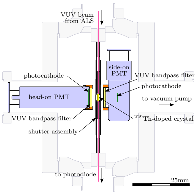
Figure 1: Experimental schematic. A ^{229}\text{Th} -doped crystal is illuminated with synchrotron radiation along its long axis. Any resulting fluorescence is collected perpendicular to this axis by a head-on type and side-on type PMT. Low-profile mechanical shutters (UniBlitz) shield the PMTs from scattered light during illumination. The assembly is held under a pressure < 10^{-5} mbar.
