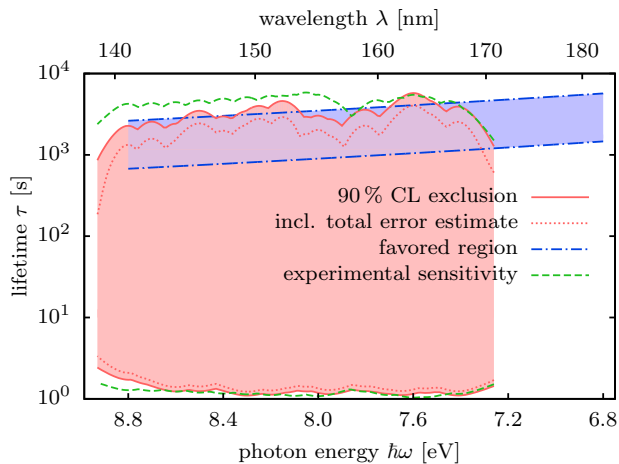
Figure 4: The 90 % CL exclusion region (red shaded) for the vacuum lifetime \tau of the ^{229}\text{Th} isomeric transition as a function of the transition energy \hbar\omega . Reduction of the sensitivity by the total error budget (Tab. II) would reduce the excluded region to the area between the red dotted lines. The experimental sensitivity (green, dashed; see text) and the favored region (blue shaded area between dash-dotted lines; see text) are also given.
