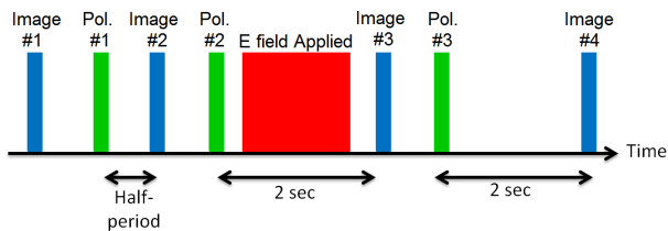
FIG. 2. (Color online) Pulse sequence used in the EDM measurement. Half-period denotes half of the spin precession period.
