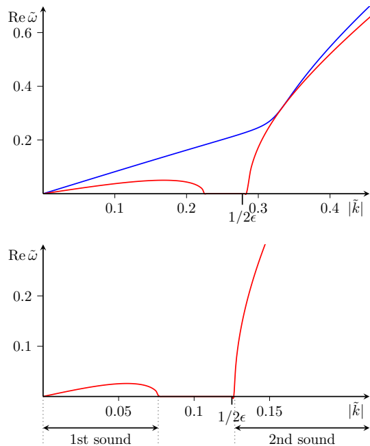
FIG. 2. Top: Small speed ratio , \epsilon < \epsilon_c . Real part of the frequency vs. |\tilde{k}| along two different directions (dotted lines of Fig.1, left). For \sin \theta > \epsilon/\epsilon_c (blue) there is no gap and a propagating mode exists at all wavelengths. On the other hand, for \sin \theta < \epsilon/\epsilon_c (red) an overdamped gap emerges, separating first sound - low \tilde{k} - from second sound - large \tilde{k} . Bottom: Large speed ratio , \epsilon > \epsilon_c . Real part of the frequency vs. |\tilde{k}| at one given value of \theta (dotted line in Fig.1, right). A non-propagating gap between first and second sound is found at any \theta . For \theta = 0 the gap extends down to k = 0 . The lower band edge of second sound occurs at \tilde{k} \sim 1/2\epsilon , that is k = \eta_0/2c_2 = k_2 , consistent with the second sound limit (8).
