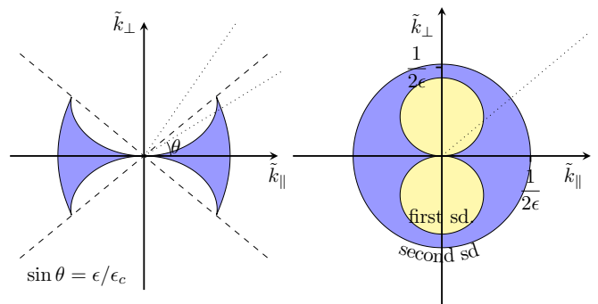
FIG. 1. Left: Small speed ratio , \epsilon < \epsilon_c . In the overdamped – nonpropagating – zone (blue) we have \text{Re } \tilde{\omega} = 0 , while in the propagating zone (white) \text{Re } \tilde{\omega} \neq 0 . The dotted lines indicate two paths along which k may be changed. The lower path, characterized by \sin \theta < \epsilon/\epsilon_c , crosses the non-propagating region, giving rise to a gap (Fig.2, top, red line). The overdamped region just touches the dashed lines marking \sin \theta = \epsilon/\epsilon_c . Right: Large speed ratio , \epsilon > \epsilon_c . The two propagating zones, \text{Re } \tilde{\omega} \neq 0 , are now completely separated by an overdamped ring (blue). Any path in momentum space connecting the region of first sound propagation (yellow) with that of second sound propagation (white) must cross the overdamped ring, giving rise to a gap between first and second sound (Fig.2, bottom).
