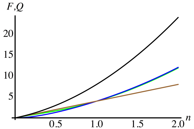
FIG. 2. Classical and quantum FIs for g = \pi/2 . in the conditional phase rotation scenario with \psi_i = (|-1\rangle + |+1\rangle)/\sqrt{2} and \psi_f = (|-1\rangle - |+1\rangle)/\sqrt{2} , and initial MA state |\alpha\rangle . Green : p_d Q_d , Blue : (1 - p_d) Q_r , Black: Q_j = 4n^2 + 4n , and Brown: Classical scaling of 4n . F_p is not shown since it is 0. The green and blue lines add up to the black line.
