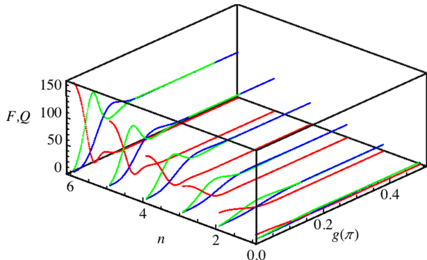
FIG. 1. Contributions to the total information from the three constituents in the conditional-phase-rotation scenario with pre- and post-selected QS state \psi_i = (|-1\rangle + |+1\rangle)/\sqrt{2} and \psi_f = (|-1\rangle - |+1\rangle)/\sqrt{2} , and initial MA state |\alpha\rangle . Red : F_p , Green : p_d Q_d , Blue : (1 - p_d) Q_r . The sum of three quantities F_{tot} equals Q_j , the total QFI of the joint system-meter state which is 4n^2 + 4n and n = |\alpha|^2 .
