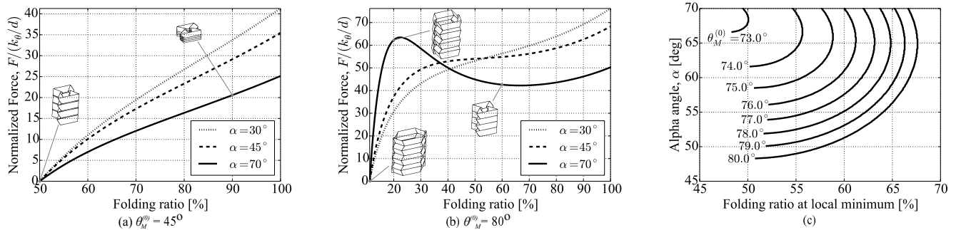
FIG. 3: Force-folding ratio relationship. The number of layers N is 7, and initial folding angle is (a) \theta_M^{(0)} = 45^\circ and (b) \theta_M^{(0)} = 80^\circ . Illustrations indicate the folded shape of the TMP with \alpha = 70^\circ . (c) Folding ratio at local minimum point under different initial angles \theta_M^{(0)} .
