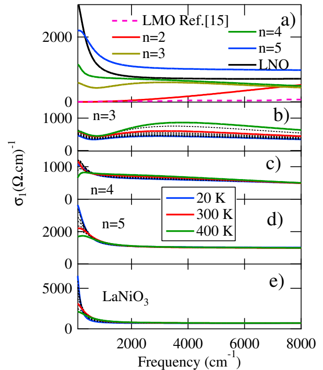
FIG. 2. Optical conductivity of the LNO/LMO superlattices as extracted from a Lorentz-Drude fitting. a) Room temperature optical conductivities of the n=2,3,4,5 samples and pure LNO and LMO. b) Temperature dependence of the optical conductivity of the n=3 compound. c-e) Same for the n=4,5 and for pure LNO.
