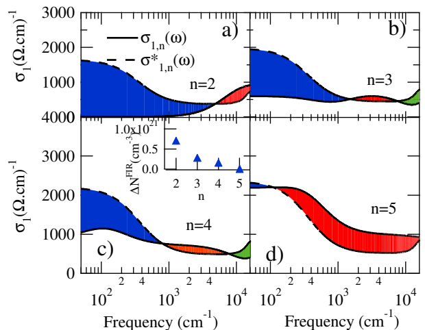
FIG. 4. Comparison between the room temperature \sigma_{1,n} , and \sigma_{1,n}^* (see text) for n=2,3,4,5 . The blue (red) area corresponds to spectral weight lost (gained) by the SL in the far- (mid-) infrared range due to the presence of interfacial effects. The green area highlights the transfer of spectral weight from higher energies.
