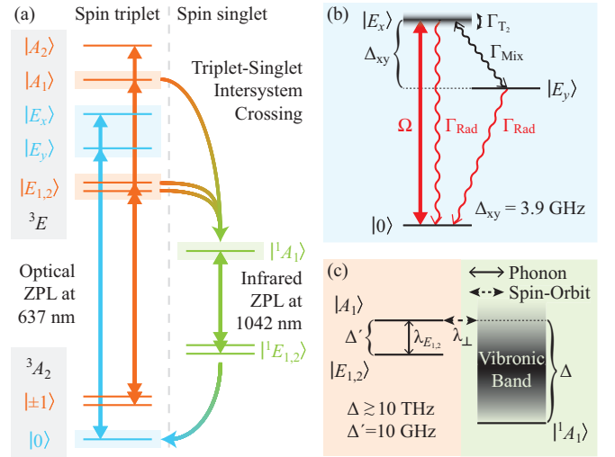
FIG. 1. The level structure of the NV center. (a) A schematic illustration of the NV center's level structure. The intersystem crossing (ISC) process is responsible for shelving into ^1E_{1,2} via the short-lived ^1A_1 and for pumping into |0\rangle . (b) The three-level system of spin-triplet, m_s = 0 states used to model phonon-induced mixing and dephasing within the ^3E manifold. (c) The states, Hamiltonian matrix elements ( \lambda_{E_{1,2}} , \lambda_{\perp} ), and energy scales ( \Delta , \Delta' ) involved in the triplet-singlet ISC.
