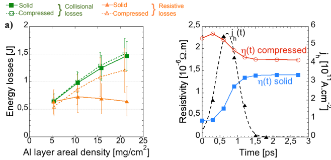
FIG. 4. (color online) Results from the hybrid transport simulations assuming \eta_{\text{laser} \rightarrow e} = 25\% : (a) Time-integrated collisional (squares) and resistive (triangles) energy losses in solid (full symbols) and compressed (open symbols) Al-samples, as a function of their areal density \rho L . (b) Time evolution of the resistivity of cold-solid (blue squares) and of warm-compressed (circles) Al samples, as well as the current beam density (triangles) averaged over a thickness of L = 35 \mu\text{m} and a radius of 25 \mu\text{m} around REB propagation axis, calculated from hybrid simulations.
