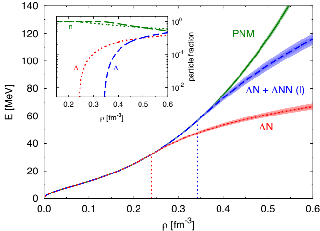
Figure 1. (Color online) Equations of state. Green solid curve refers to the PNM EoS calculated with the AV \delta^8 +UIX potential. The red dotted curve represents the EoS of hypermatter with hyperons interacting via the two-body \Lambda N force alone. The blue dashed curve is obtained including the three-body hyperon-nucleon potential in the parametrization (I). Shaded regions represent the uncertainties on the results as reported in the text. The vertical dotted lines indicate the \Lambda threshold densities \rho_{\Lambda}^{th} . In the inset, neutron and lambdas fractions corresponding to the two HNM EoSs.
