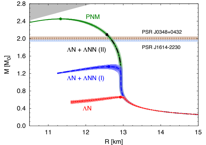
Figure 2. (Color online) Mass-radius relations. The key is the same of Fig. 1. Full dots represent the predicted maximum masses. Horizontal bands at \sim 2M_{\odot} are the observed masses of the heavy pulsars PSR J1614-2230 [18] and PSR J0348+0432 [19]. The grey shaded region is the excluded part of the plot due to causality.
