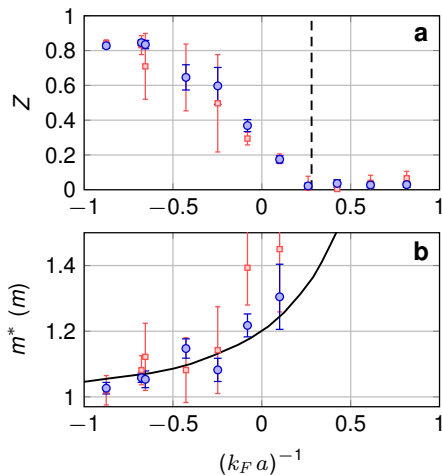
FIG. 3. Z and effective mass. a , The quasiparticle spectral weight Z decreases as (k_F a)^{-1} increases. Using a linear fit to the range -0.5 \leq (k_F a)^{-1} \leq 0.3 , we find that Z vanishes at (k_F a)^{-1} = 0.28 \pm 0.02 (dashed line); this marks the breakdown of a Fermi liquid description. The blue circles come from fits of a large range of data, from 0 to 1.5 k_F . The red squares show the result of restricting the fit to 0.7 to 1.3 k_F , and they show a similar trend and slightly larger error bars. b , The quasiparticle effective mass m^* is shown for the region where Z > 0 . Interactions increase m^* , and the data (circles) agree surprisingly well with the theoretical prediction for the limiting case of the Fermi polaron (solid line)[10, 30]. Restricting the fit to EDCs close to the Fermi surface produces similar results with increased error bars (red squares).
