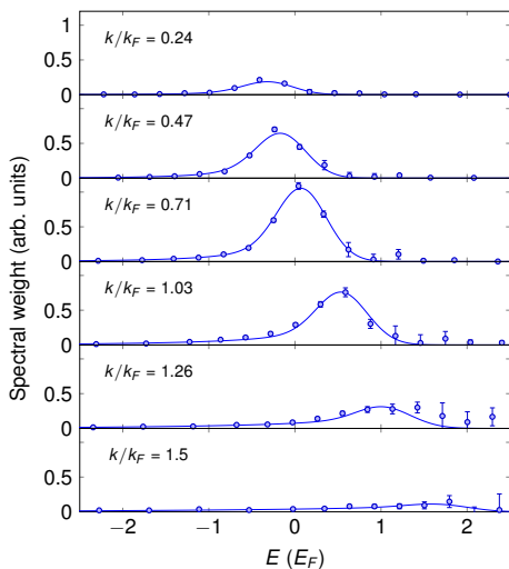
FIG. 2. EDCs for atom PES data near unitarity. Data (circles) and fits (lines) are shown for several example traces at fixed k through the PES data at (k_F a)^{-1} = -0.08 . These traces are often called energy distribution curves, or EDCs. Here, the fitting parameters are Z = 0.37 \pm 0.03 , m^* = 1.22 \pm 0.03 , T = 0.24 \pm 0.02 , E_0 = -0.33 \pm 0.02 , \mu = 0.19 \pm 0.04 , E_p = 0.23 \pm 0.04 , T_p = 1.09 \pm 0.08 , where the error margins are for one standard deviation and also include a 5% uncertainty in E_F . For this fit, the reduced \chi^2 is 1.2.
