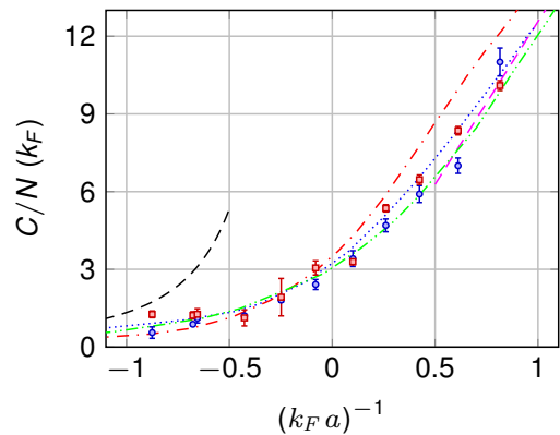
FIG. 4. The contact parameter. From the PES data, we extract the contact per particle (in units of k_F ) for a homogeneous Fermi gas above T_c as a function of the interaction strength (k_F a)^{-1} . The contact measured from the tail of the rf lineshape[24], using data for h\nu \geq 5E_F , is shown in blue circles, while the contact extrapolated from the fits of the PES data is shown in red squares. Remarkably, even though we limited the fits of the PES data to k \leq 1.5 and E \geq -3 , a region with a relatively small contribution of short-range correlations [21, 26, 27, 36], we find that the contact from the PES fits is consistent with the contact measured from the tail of the momentum-integrated rf line shape. For comparison with the data, we also plot the BCS (dashed black line) and BEC (dashed magenta line) limits, given by 4(k_F a)^2/3 and 4\pi(k_F a)^{-1} , respectively [27], the non-self-consistent t-matrix at T = 0 (dotted blue line) and its Popov version at T_c (dash-dotted red line) [38], and the self-consistent t-matrix model at T = 0 (double-dotted green line) [18]. Interestingly, we find that the contact measured above T_c agrees well with the T = 0 theories.
