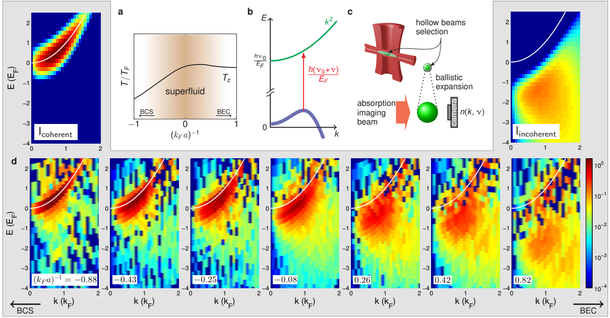
FIG. 1. Atom PES data. a , We take data above T_c in the strongly interacting region of the BCS-BEC crossover[19]. After initially preparing the gas at small, positive a , the magnetic field is swept adiabatically to a final value within the BCS-BEC crossover, where |(k_F a)^{-1}| < 1 . b , Schematically, an rf photon, which has a negligible momentum, transfers an atom from the strongly interacting state (blue line) to a weakly interacting state (green line). The energy and momentum of the atom in the strongly interacting state are extracted from the measured momentum of the spin-flipped atom and the rf detuning \nu [13]. The detuning, \nu , of the rf frequency is varied to obtain data for a wide range of E and k . c , Immediately following the rf pulse and before time-of-flight expansion, two orthogonally propagating hollow-core beams optically pump atoms at the edges of the outcoupled atom cloud into a dark state [20, 21]. The durations of both the rf pulse and optical pumping are short compared to motion of atoms in the trap. d (lower panel) , In these example plots of PES data, the color represents the probability distribution of atoms at a given E and k in the strongly interacting gas. We estimate that the error bar of (k_F a)^{-1} is 0.03. E = 0 is the energy of a free atom at rest and the white line shows the free-particle dispersion E = k^2 . d (upper panel) , Our two-mode fit function includes a fermionic quasiparticle part, shown on the left with m^* = 1.05 , E_0 = -0.1 , \mu = 0.5 , and T = 0.25 , and an incoherent part, shown on the right with E_p = 1.5 and T_p = 0.7 .
