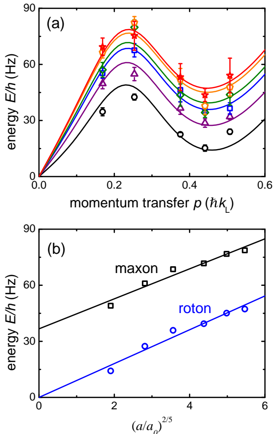
FIG. 3: (Color online) Roton/maxon energy vs. scattering length. (a) We measure the excitation spectra at different scattering lengths a/a_0 = 5(\circ), 13(\triangle), 24(\square), 40(\diamond), 55(\circ) and 70(\star) . The condensate number is N_0 = 9,000 . Solid curves are fits based on Eq. (1). A global optimization procedure gives V = 6.7(2) E_R and \Delta x = 43(3) nm. (b) Roton energies ( \circ ) and maxon energies ( \square ) extracted from the fits in panel (a) are shown at different scattering lengths. Solid curves are fits based on \Delta_r = A(a/a_0)^{2/5} and \Delta_m = B + C(a/a_0)^{2/5} , from which we obtain A = h \times 9(1) Hz, B = h \times 37(9) Hz and C = h \times 8(1) Hz.
