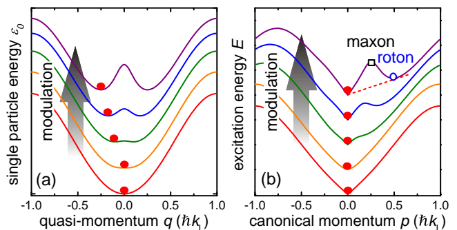
FIG. 1: (Color online) Generation of roton-maxon dispersion in a shaken lattice. (a) For a single atom, the lattice modulation creates a double-well structure above a critical modulation amplitude (top three lines) [21]. In our experiment, the atoms are prepared at the minimum with zero or negative momentum ( q^* \leq 0 , red dot); see text. (b) With atomic interactions, a roton minimum (o) and a maxon maximum (□) in the excitation spectrum can form. The dashed line indicates the critical velocity limited by the roton minimum according to the Landau criterion for superfluidity. Dispersions are upward offset with increasing modulation amplitude for clarity. The lattice reciprocal momentum is \hbar k_L = h/\lambda where \lambda is the wavelength of the lattice beams and h = 2\pi\hbar is the Planck constant.
