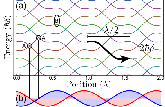
FIG. 1: (color online) Part (a) shows the eigenvalues of the two-frequency dressed state system separated by \hbar\delta where the two fields have equal strength, along with a typical path followed by an atom moving to the right. Circled transition points of the type marked “A” are exact crossings because they occur at the nodes of the standing wave fields shown in part (b). For our case this occurs for a spatial phase offset of \lambda/8 and \Omega = \sqrt{3/2} \delta . Point “B” in the vertical ellipse marks the location of a possible Landau-Zener transition.
