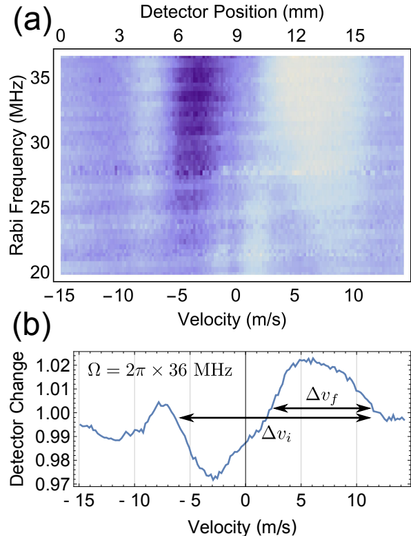
FIG. 3: (color online) Data taken with an optical slit width \approx 230 \mu\text{m} corresponding to interaction time of 220 \text{ ns} < t_{SE} for longitudinal velocity \approx 1050 \text{ m/s} . The detuning was \delta = 2\pi \times 25 \text{ MHz} corresponding to \Delta v_B \approx 4.9 \text{ m/s} . In part (a) the dark regions represent reduced atomic intensity and the lighter regions increased intensity. The image has been corrected for detector inhomogeneity as discussed in the text. Part (b) shows a profile taken near the top of part (a) at \Omega \approx 2\pi \times 36 \text{ MHz} . The initial ( \Delta v_i ) and final velocity widths ( \Delta v_f ) are indicated.
