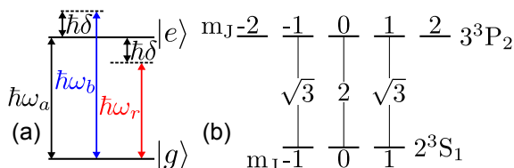
FIG. 2: Part (a) shows the two atomic levels and the detuning \delta \gg \gamma . Part (b) shows the \Delta m = 0 transitions driven by the linearly polarized light between the J = 1 and J = 2 He levels and their relative strengths.
