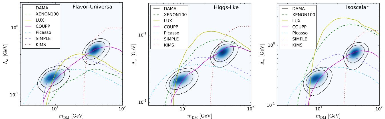
FIG. 1. 2-dimensional credible regions for DAMA (shaded/black solid, 90% and 99% CL) and exclusion limits (99.5% CL) in the (m_{\text{DM}}, \Lambda_a) plane, for flavor-universal (left), Higgs-like (center) and isoscalar (right) couplings.
