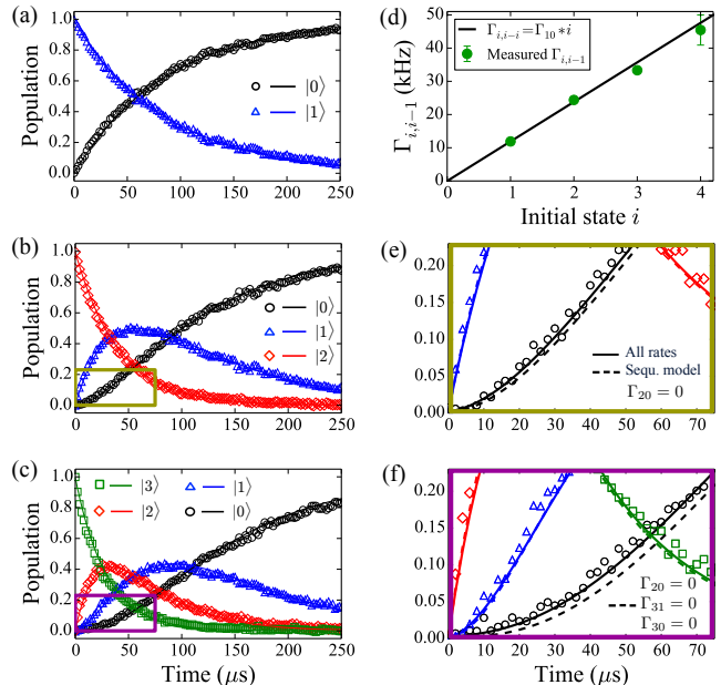
FIG. 2. (a)-(c) Population decay traces of the qubit states up to |3\rangle , obtained by varying the time delay \Delta t before the depopulation sequence. The solid lines are state occupations from the multi-level decay model taking into account all decay channels. (d) The sequential decay rates \Gamma_{i,i-1} (green dots) for increasing energy state i , showing the roughly linear dependance (solid line). (e)(f) Zoom of decay curves in panel (b) and (c) respectively, showing the model with all transition rates allowed (solid line) compared to the model with only neighboring transitions allowed (dashed line). The extracted decay times are listed in Tab. I.
