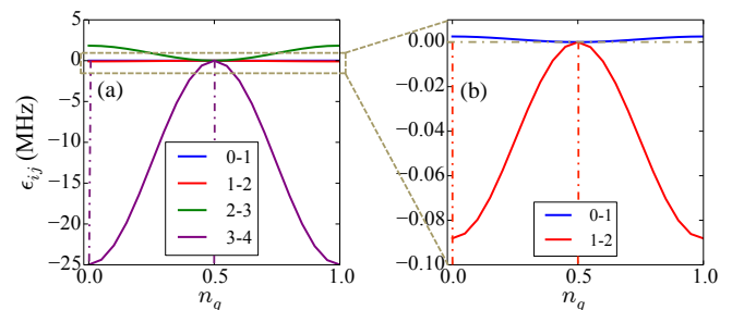
FIG. 4. (a) Calculated change in transition frequency \epsilon_{ij}(n_g) as a function of the effective offset charge n_g , expressing the charge dispersion of each transition. (b) Zoom of the lowest two transitions 0-1 and 1-2.
