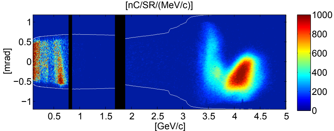
FIG. 5. Energy spectrum of a 4.2 GeV electron beam measured using the broadband magnetic spectrometer. The plasma conditions closely match those in Fig. 2(c). The white lines show the angular acceptance of the spectrometer. The two black vertical stripes are areas not covered by the phosphor screen.
