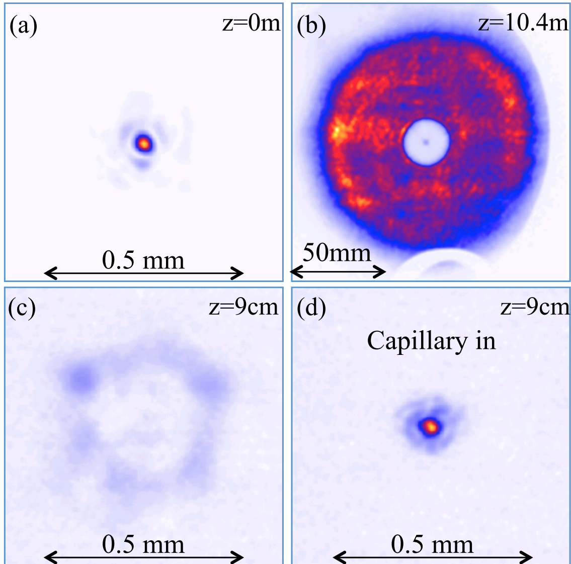
FIG. 1. Typical laser spatial profiles in vacuum with laser energy 16 J for (a) focus, (b) z=10.4 m downstream of focus, and (c) z=9 cm downstream of focus. The near-field (b) shows an approximately top-hat profile. In (d) the guided mode is shown for plasma density 7.5 \times 10^{17} \text{ cm}^{-3} . Well-confined high-quality modes were observed for density as low as 2 \times 10^{17} \text{ cm}^{-3} . The color scale is the same for (c) and (d).
