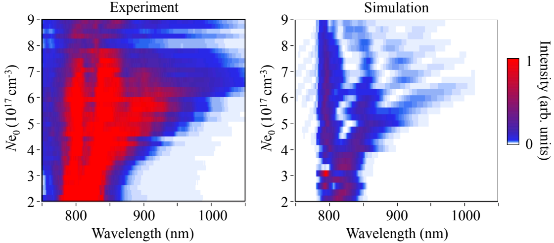
FIG. 3. Measured (left) and simulated (right) optical spectra at the output of the 500 \mu\text{m} diameter capillary as a function of plasma density for input laser energy \approx 7.5 \text{ J} and pulse duration \approx 40 \text{ fs} . The spectral response of the detection system was applied to the simulated data.
