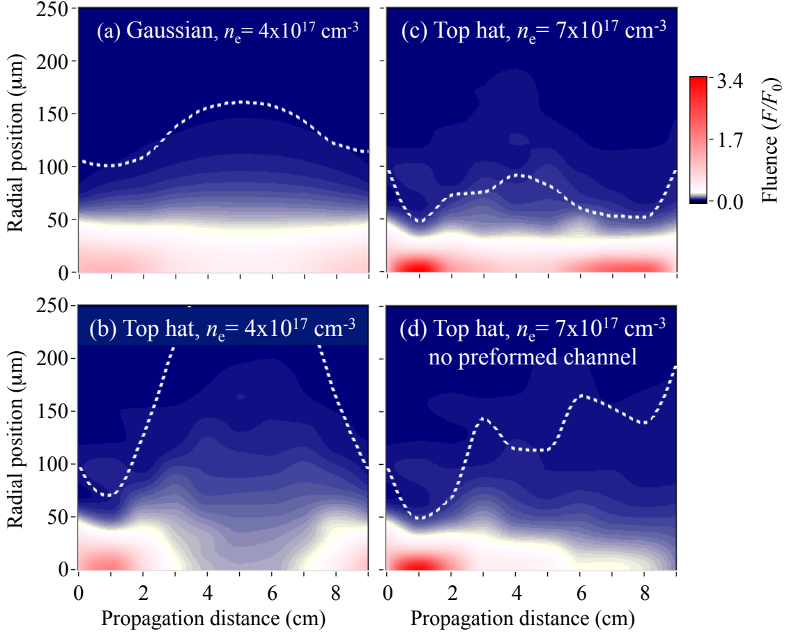
FIG. 2. Laser pulse radial fluence profile evolution through the waveguide for different plasma density and initial fluence profiles for input laser energy 15 J. In each image the color scale represents the fluence (each normalized to the peak fluence at z = 0 ) and the dashed line is the diameter at which the fluence drops to 1/e^2 of the on-axis value. For (a) the initial laser pulse radial profile is Gaussian and the preformed channel is defined by r_m = 81 \mu\text{m} and n_e(0) = 4 \times 10^{17} \text{cm}^{-3} . In (b), (c), and (d) the near-field of the laser pulse has a top-hat profile. For the same density and channel depth as in (a), (b) shows that the guiding is less efficient for the top-hat case. For (c) the combination of self-guiding and preformed plasma channel ( r_m = 81 \mu\text{m} ) mitigates diffraction over the full length of the plasma. Without a preformed plasma channel (d) self-guiding reduces the laser spot size for the first 2 cm but the laser diffracts strongly before the exit of the channel.
