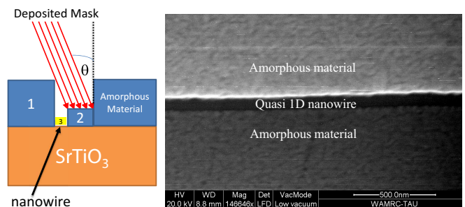
FIG. 1: (color online). (Left panel) Fabrication method of the nanowires. On top of \text{TiO}_2 terminated \text{SrTiO}_3 substrate an amorphous oxide layer number 1 with a thickness d was deposited and patterned with standard optical lithography process. The substrate is then tilted to an angle \theta and a second amorphous oxide layer is deposited. This results in a nano-trench with a width w = d \tan(\theta) . Finally an epitaxial \text{LaAlO}_3 layer is deposited as described in the text resulting in a conducting \text{LaAlO}_3/\text{SrTiO}_3 nanowire. Right panel: Scanning electron microscope image of such nanowire designed with w = 70\text{nm} consistent with the dimensions measured by the microscope.
