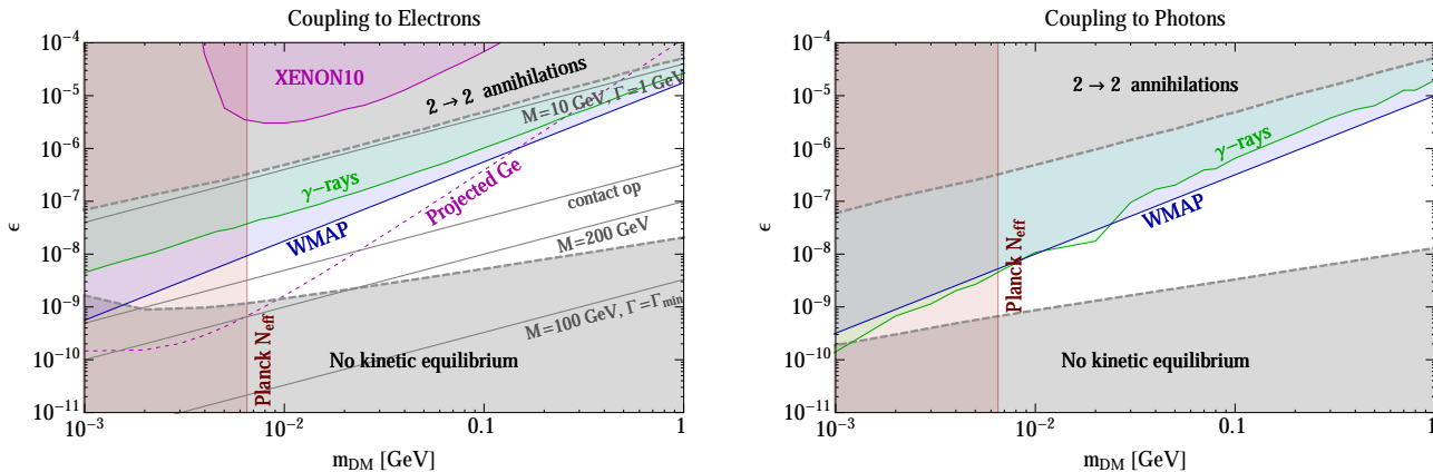
FIG. 3: The bounds on \epsilon vs. m_{\text{DM}} . In both panels, the grey regions (outlined by thick dashed lines) represent the range of parameters in which kinetic equilibrium with the SM is not maintained (lower gray region), and where the standard 2 \rightarrow 2 annihilation to the SM is not subdominant to the 3 \rightarrow 2 process (upper gray region). Left, coupling to electrons: Additional exclusion limits from: direct-detection in Xenon10 (purple region), and the expected future bound from a germanium-based electron recoil experiment (dashed-purple); CMB and low red shift data constraints for electrons (blue region); modification of N_{\text{eff}} (red region); indirect detection of \gamma -rays (green region); direct production at LEP for a variety of mediator mass, M , and width, \Gamma (solid-gray). Right, coupling to photons: Additional exclusion limits from: indirect detection of \gamma -rays (green region); conservative CMB and low red shift data constraints (blue region); modification of N_{\text{eff}} (red region).
