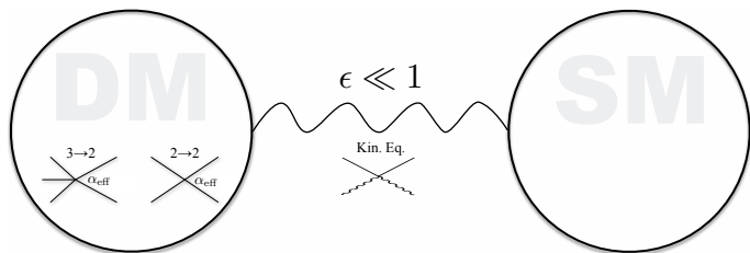
FIG. 1: A schematic description of the SIMP paradigm.
