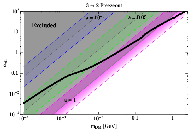
FIG. 2: \alpha_{\text{eff}} vs. DM mass (black solid line), derived from the numerical solution to the Boltzmann Equation in the 3 \rightarrow 2 freeze-out scenario. The colored regions show the preferred region for the ‘core vs. cusp’ and ‘too-big-to-fail’ anomalies for a = 1 (magenta), a = 0.05 (green), and a = 10^{-3} (blue). The region above the gray-dashed lines is excluded by the bullet-cluster and halo shape constraints, for each value of a .
