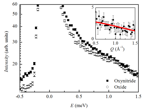
FIG. 5. E -cuts of the oxide and oxynitride neutron scattering spectra at 1.5 K ( Q = [0.5, 2.0] \text{ \AA}^{-1} ). Inset: Q -dependence of the background subtracted inelastic scattering from the oxynitride sample at the same temperature, to which an F(Q)^2 form was fitted (solid line).
