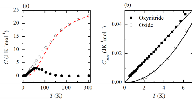
FIG. 1. (a) Total heat capacity C of \text{Lu}_2\text{Mo}_2\text{O}_7 (open circles) with the estimated lattice (dashed line) and magnetic C_{mag} (closed circles) contributions. (b) The magnetic heat capacities of the oxide and oxynitride phases.
