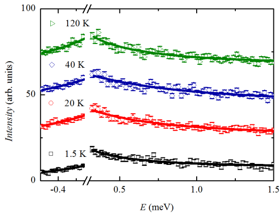
FIG. 4. Offset E -cuts ( Q = [0.5, 2.0] \text{ \AA}^{-1} ) for the oxynitride sample at various temperatures with fits (solid lines) of Eqn.2 to the data.
