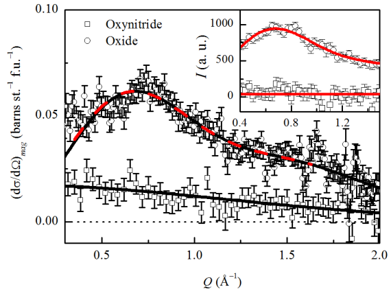
FIG. 2. The magnetic scattering cross sections of the both samples at 1.5 K. The solid lines are fits to the data. The inset shows the elastic magnetic scattering measured on CNCS at 1.5 K. A scaled version of the fit of Eqn.1 to the CNCS oxide data is shown on top of the D7 data (dashed line).
