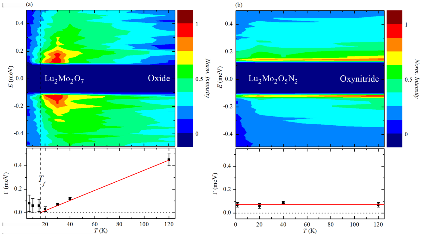
FIG. 3. The temperature dependence of background subtracted, normalised inelastic neutron scattering ( Q = [0.5, 2.0] \text{ \AA}^{-1} ) (top) and the energy width of the inelastic spectra, \Gamma , (bottom) for the (a) oxide and (b) oxynitride, respectively.
