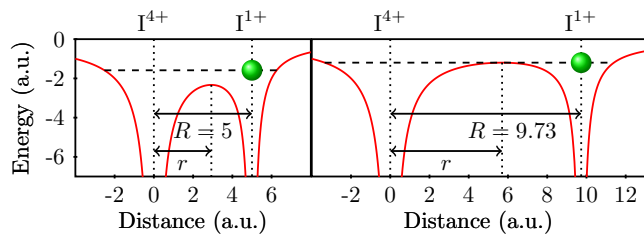
FIG. 4. Illustration of the COB model for the coincidence channel (1,4). At R_{\text{eq}} = 5 a.u. the most loosely bound electron ( E_{P_f} = -19.2 eV [21]) can easily overcome the potential barrier towards I^{4+} while electron transfer is blocked beyond R_{\text{crit}} = 9.73 a.u..
