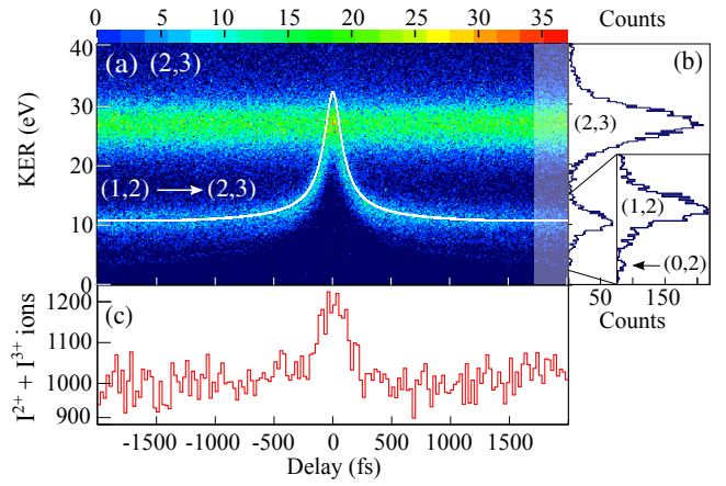
FIG. 2. (a) KER for all coincident (2,3) ion pairs plotted as a function of the time delay. The classical simulation via the pathway (1,2) \rightarrow (2,3) is superimposed in white. (b) Projection of KERs at large delays (shaded area) onto the KER axis with the inset showing a magnified view of the low-energy region. The charge states belonging to the observed asymptotic KERs are indicated in brackets. (c) Projection of all KERs onto the delay axis.
