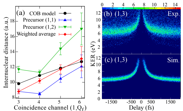
FIG. 5. (a) R_{\text{crit}} as a function of the asymmetric coincidence channel (1, Q_f) with Q_f \in \{3, 4, 5, 6\} . The black circles show the predictions from the COB model R_{\text{crit}}^{\text{COB}} with E_{P_f} = -19.2 eV [21], while the experimental data R_{\text{crit}}^{\text{exp}} for the precursor (1,1) are drawn as blue upwards triangles, those for (1,2) as green downwards triangles and the weighted average as red diamonds. (b) Delay-dependent KER for (1,3). (c) Simulation of the delay-dependent KER for (1,3) with a finite pulse length of 57 fs (FWHM) and a width for the spatial ground state distribution of 0.5 a.u. (FWHM).
