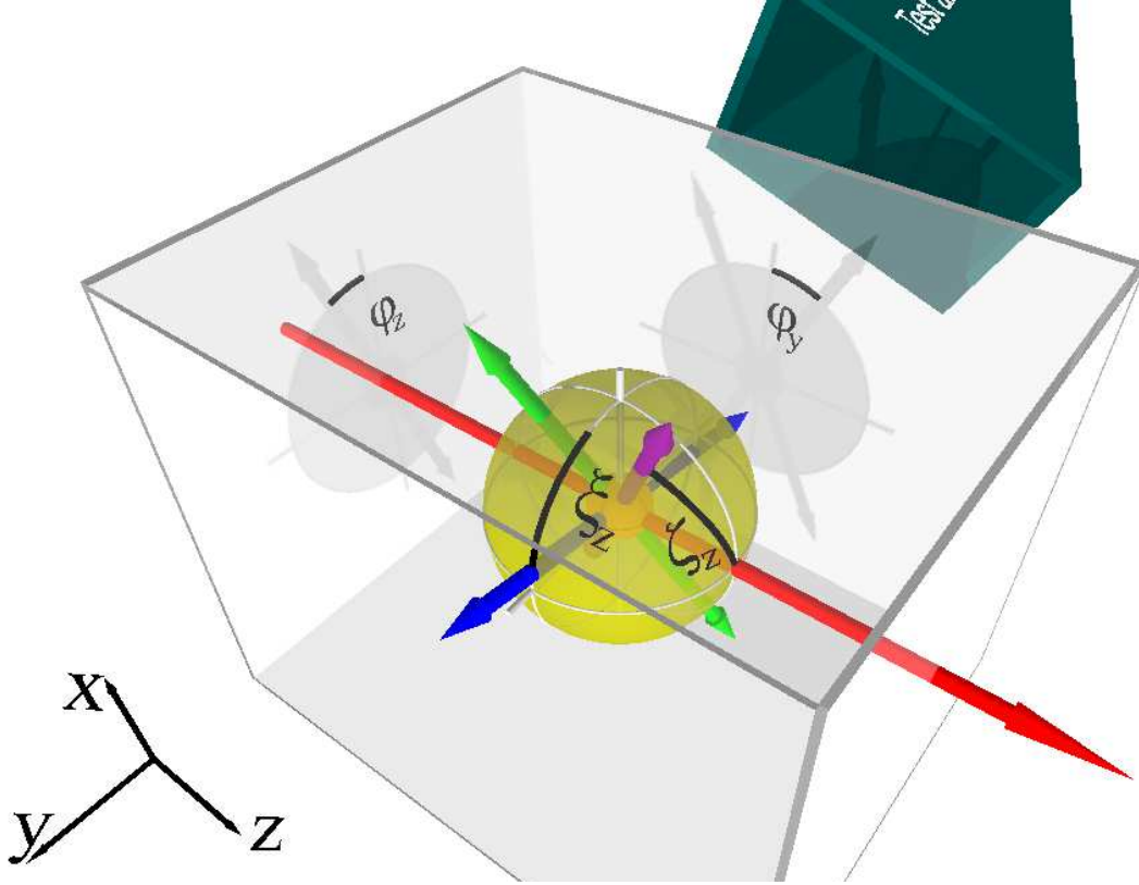
FIG. 3. (Color online) Schematic view of the setup including the cell in the foreground and the test antenna in the background. The laser propagation direction (red), the polarization of the two laser beams (blue) and an arbitrary polarization direction of the MW (magenta) are shown together with the relevant angles between them as described in the main text. The shadows are the projections onto the \hat{x} - \hat{y} plane on the left and the \hat{x} - \hat{z} plane in the back.
