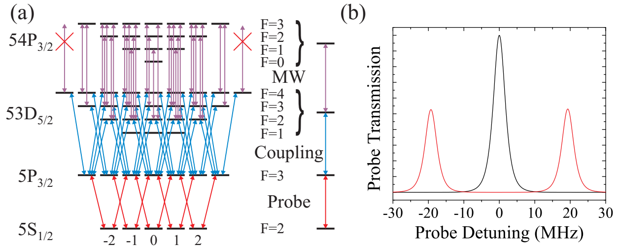
FIG. 1. (Color online) (a) Level diagram showing all 52 possible states addressed by the experiment. The arrows indicate allowed excitations for \sigma polarized probe and coupling beams and \pi polarized MW's. The 54P_{3/2} states are shown above the 53D_{5/2} states for simplicity. On the right, the corresponding effective 4-Level system is shown. (b) Theoretical lineshapes resulting from a 3-level (black) and 4-level (red) system.
