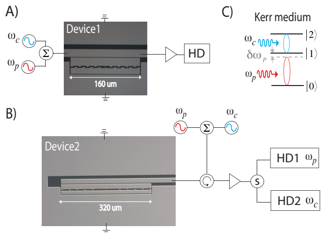
FIG. 1: A micrograph of Device 1 in A) and Device 2 in B) with measurement setup using heterodyne detection (HD). Device 1 and 2 have an artificial atom, a transmon qubit, embedded in a 1D open transmission line and at the end of a transmission line, respectively. In B), we measure the reflection coefficient of the probe and control fields simultaneously. C) The three-level artificial atom driven by a probe (red) and a control tone (blue). The artificial atom acts as a Kerr medium, which enables photon-photon interaction.
