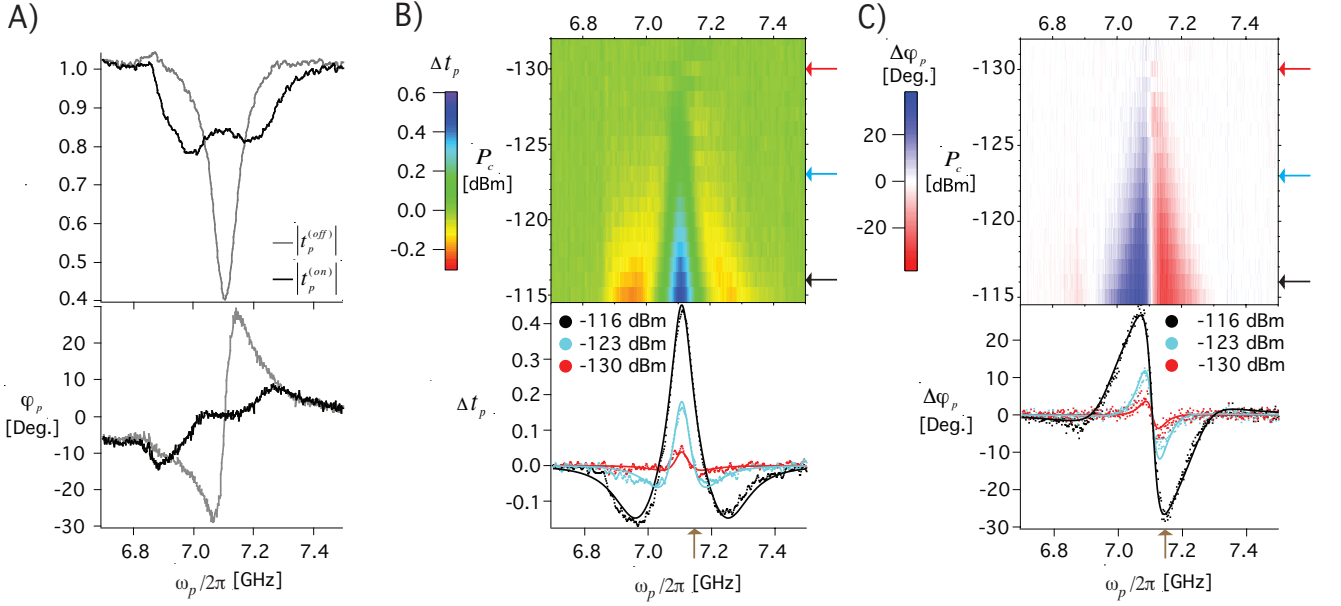
FIG. 2: Transmission coefficient for the probe, as a function of \omega_p and control power, P_c , for low probe powers, \Omega_p \ll \gamma_{10} in Device 1 (see the Supporting Online Material (SOM) for Device 2). (A) Top: Measured transmission coefficient with P_c = -116 dBm, |t_p^{(on)}| (black), and P_c turned off, |t_p^{(off)}| (grey). Bottom: corresponding phase response. (B) Measured amplitude response, \Delta t_p . (C) Measured phase response, \Delta\varphi_p . Top panels: as a function of probe frequency and control power. Bottom panels: horizontal line cuts (dots) and theory curves (solid lines). Brown arrows show the frequency that maximizes the phase response. The theory curves [24, 25] are fit simultaneously to extract \gamma_{20}/2\pi = 150 MHz along with the control field coupling. The following other parameters, also used in the calculations, are independently measured with single-tone and two-tone spectroscopy: \omega_{10}/2\pi = 7.10 GHz, \omega_{21}/2\pi = 6.38 GHz, \Gamma_{10}/2\pi = 74 MHz, \gamma_{10}/2\pi = 60 MHz and the probe field coupling.
