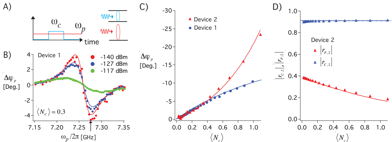
FIG. 3: Probe phase shift, \Delta\varphi_p , induced by a weak control pulse. Solid curves are theoretical fits to the data, including additional data in the SOM. The fitting parameters for each device are \gamma_{20} and the control field coupling. Other parameters are measured independently through spectroscopy. All parameters are listed in Table I. (A) The control pulse induces a phase shift, \Delta\varphi_p , of the continuous probe in the time domain. The length of the pulse is 1 \mu\text{s} for device 1 and 7 \mu\text{s} for device 2. (B) \Delta\varphi_p as a function of \omega_p for three different probe powers and \langle N_c \rangle \simeq 0.3 , for Device 1. Note that here the |0\rangle \leftrightarrow |1\rangle transition is 7.26 \text{ GHz} (due to a different external magnetic flux, \Phi ). (C) \Delta\varphi_p as a function of \langle N_c \rangle for a weak probe at a probe frequency that maximizes the probe phase shift. Each data point is an average over 2 million control pulses. An average phase shift of 10 degrees per control photon is observed in Device 1, and 20 degrees per control photon in Device 2. (D) |r_{p,2}| and |r_{c,2}| as a function of \langle N_c \rangle . The dashed blue line indicates |r_{c,2}| = 0.9 . Extensive measurements of r_{p,2} are presented in Fig. S4A of the SOM.
