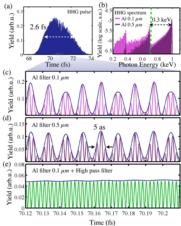
FIG. 2. (a) Detailed structure of an X-ray burst from the trailing edge of the keV pulse train shown in Fig. 1. The spectrum of the selected burst is shown in (b) for Al filters of 0.1 and 0.5 \mu\text{m} thickness. Plots (c) and (d) show a magnification of the temporal structure for the two Al filters respectively, whereas (e) corresponds to the X-ray field obtained by selecting only the highest frequency contributions to the spectra.
