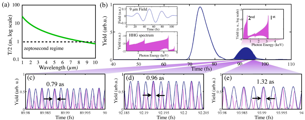
FIG. 3. (a) Predictions for the width of each keV beat in the waveform ( T/2 ) as a function of the laser wavelength. (b) Envelope of the X-ray bursts obtained from a 1.5-cycle midIR pulse with wavelength \lambda = 9 \mu\text{m} . Left insets: electric field of the driving pulse and high-harmonic spectrum. Right inset: spectral content of the second fs burst. Panels (c) to (e) detail the fine temporal structure of the second fs burst: (pink line) absolute value of the electric field, and (dark blue line) field envelope.
