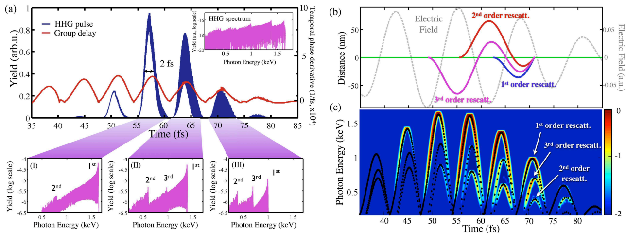
FIG. 1. (a) Envelope of the X-ray bursts (blue line) and group delay (red line) obtained using a 3.9 \mu\text{m} wavelength laser. The HHG spectrum is shown in the inset, while in the panels below the spectral content of each burst is shown. (b) Schematic of the driving field and an example of the interfering trajectories contributing to the fs burst at 71 fs. (c) Time-frequency analysis (logarithmic scale). The dotted lines represent classical calculations of the electronic rescattering energies of trajectories with different rescattering orders.
