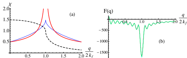
FIG. 2: (a) The static spin susceptibility \chi(q) as a function of momentum for a FL (dashed, black) and the gauge-fermion model with \sigma < 1/3 (dotted, blue) and \sigma > 1/3 (solid, red). (b) F(q) as a function of momentum for angles \theta = 0, \pi/6, \pi/4 . The curves for different angles are almost identical. Here the spins form a square lattice, and \sigma = 1/2, k_F a = 0.2 .
