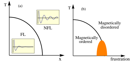
FIG. 1: Schematic electronic (a) and magnetic (b) phase diagrams for a Kondo lattice model with strongly interacting conduction electrons coupled to localized spins. (a): Crossover from FL to NFL behavior. x represents non-thermal tuning parameter, e.g. pressure, magnetic field, doping. Distance dependence of RKKY interaction is shown in the insets. (b): Magnetic transition temperature decreases with increasing frustration resulting from NFL-mediated longer-range RKKY interaction. New phases (shaded region), e.g. a glass phase, emerge near the putative QCP.
