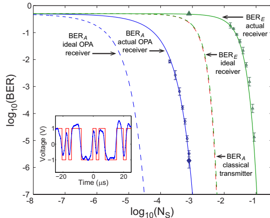
FIG. 2: (color). \text{BER}_A and \text{BER}_E versus source brightness N_S for 500 kbit/s communication. Inset: 25 bits of OPA-receiver detector output (blue) and Bob’s corresponding modulation waveform (red). See text for more information.
