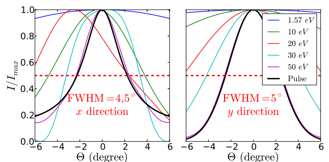
FIG. 2. (color online) Far field angular distribution at a range of photon energies. The asymmetry in the left panel ( x -direction) is due to the oblique incidence. The right panel shows polarization- ( y -) direction. Profiles are taken at 1 \text{ mm} distance from the cone. The thick black lines show divergence for a pulse composed of all harmonics above 45 \text{ eV} .
