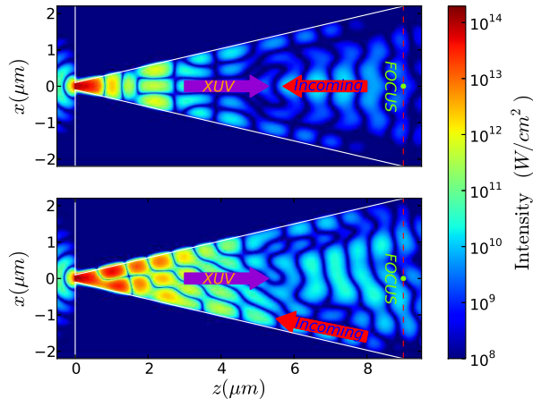
FIG. 1. (color online) Simulation results: intensity distribution in the silver cone in the xz -plane at peak plasmon field of 2 \times 10^{14} \text{ W/cm}^2 . Normal (upper panel) and oblique incidence (lower panel). Polarization is in y -direction perpendicular to the plane. Oblique incidence angle is 7 degrees in the xz -plane parallel to the inner cone surface. In both cases, the harmonic beam is emitted in the direction of the cone axis.
