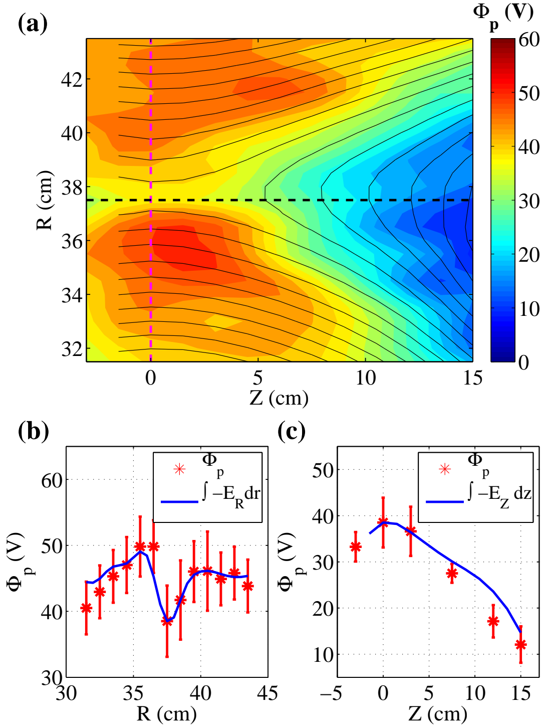
FIG. 2. (a) Measured 2-D plasma potential profile with contours of the poloidal flux \Psi . The radial potential well becomes deeper and wider downstream. (b) Radial profile of \Phi_p at Z = 0 (along the magenta dashed line in (a)). The red asterisks are the measured \Phi_p and the blue line is the radial integration of the right-hand side of Eqn. (2). Two profiles are in agreement. (c) Axial profile of \Phi_p at R = 37.5 cm (along the black dashed line in (a)). The red asterisks are the measured \Phi_p and the blue line comes from the integration of the right-hand side of Eqn. (4) along Z .
