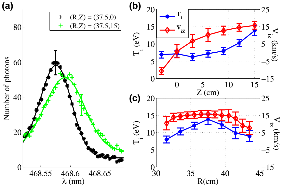
FIG. 4. (a) Spectra of He 4686 Å at (R, Z) = (37.5, 0) (black) and at (R, Z) = (37.5, 15) (green). Solid lines are from fitting the spectra into the sum of 13 Gaussian functions. Both ion heating and acceleration are observed at (R, Z) = (37.5, 15) . (b) Axial T_i and V_{iZ} profiles at R = 37.5 cm. For Z > 9 cm, the ion temperature rises significantly while V_{iZ} begins to saturate. (c) Radial T_i and V_{iZ} profiles at Z = 15 cm (downstream). The ion temperature profile is peaked at the center of the layer while the outflow profile is broader.
