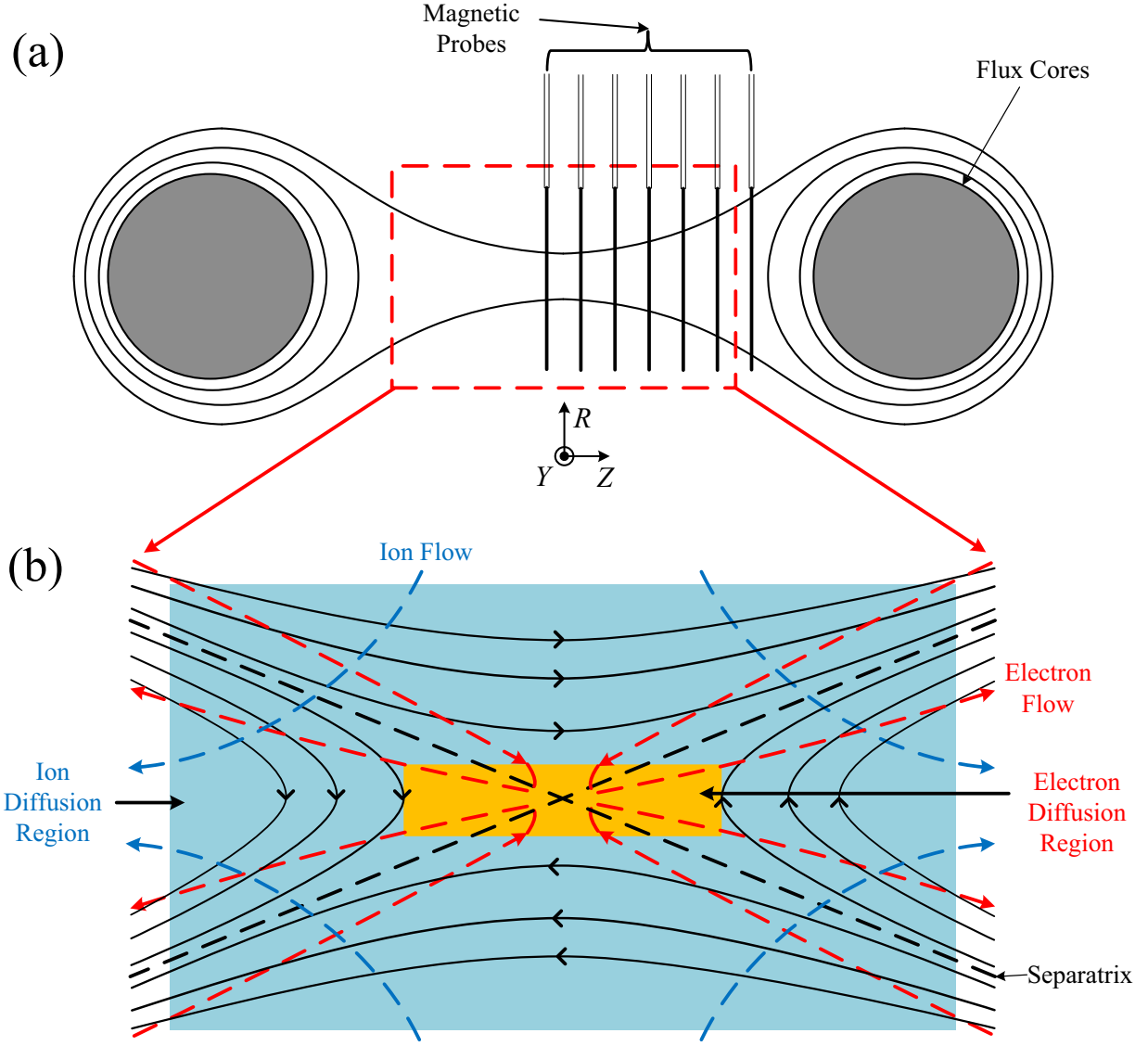
FIG. 1. (a) A cross section of MRX. The flux core contains the PF coil for driving magnetic reconnection and the TF coil for creating the plasma. Magnetic probes are inserted to monitor the evolution of the 2-D magnetic geometry. (b) Enlarged view of the reconnection layer marked by the dashed red box in (a). The electron diffusion region (EDR) is embedded in the much larger ion diffusion region (IDR). The blue dashed lines illustrate typical ion flow, while the red lines show electron flow.
