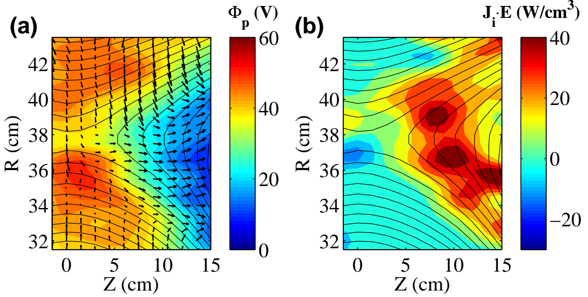
FIG. 3. (a) In-plane ion flow vector measured by Mach probes together along with contours of \Phi_p and \Psi . The flow vectors are measured every 1 cm along R and every 3 cm along Z . The maximum ion velocity is 16 km/s. As ions flow across the separatrices, they are accelerated by \mathbf{E}_{in} and turn into the outflow direction. (b) Work done by the electric field on ions. It is dominated by the strong Hall field.
