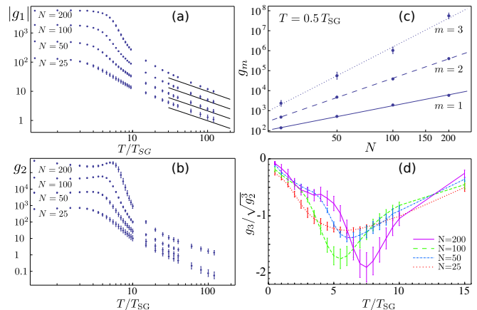
FIG. 1: MC data for the statistics of the mesoscopic conductance fluctuations at different temperatures and system sizes. In panel (a) shown is the average conductance g_1 as a function of temperature. The asymptotes given by Eq. (20) are shown for comparison as solid black lines. Panel (b) shows the second cumulant g_2 of the conductance distribution. Panel (c) shows the dependence of the first three cumulants at T = 0.5 T_{\text{SG}} on the system size. The log-log plot shows a good fit with the g_m \sim N^{m+1} scaling. Panel (d) shows the skewness of the distribution of conductance values as a function of temperature.
