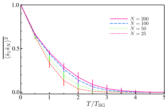
FIG. 2: Spin-spin correlation function at the opposite ends of the sample as a function of temperature for various systems sizes. Note that larger system sizes result in stronger correlations at given temperature. This effect is caused by the long-rangedness of the RKKY exchange resulting in the logarithmic renormalization of the spin-spin interaction constant with increasing system size.
