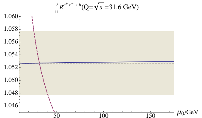
FIG. 1: The final PMC result for R^{e^+e^- \rightarrow h} as a function of the initial renormalization scale \mu_0 (solid blue line), demonstrating the initial scale-invariance of the final prediction, up to strongly suppressed residual dependence. The shaded region is the experimental bounds with the central value given by the thin dashed line. For comparison we also show the pQCD prediction before PMC scale setting (dashed red line) fixed to the experimental value for \mu_0 = Q . This result is very sensitive to \mu_0 , and is thus severely violating the renormalization group properties.
