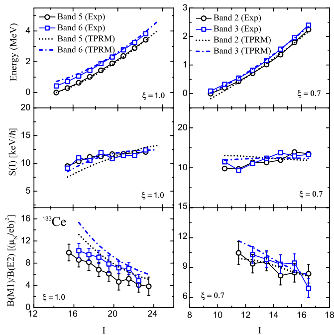
FIG. 2: (Color online) Experimental excitation energies, S(I) parameters, and B(M1)/B(E2) ratios for the negative-parity chiral doublet (left panels) and positive-parity chiral doublet (right panels) in ^{133}\text{Ce} . Also shown are results of TPRM calculations with the indicated attenuation factors \xi (see text).
