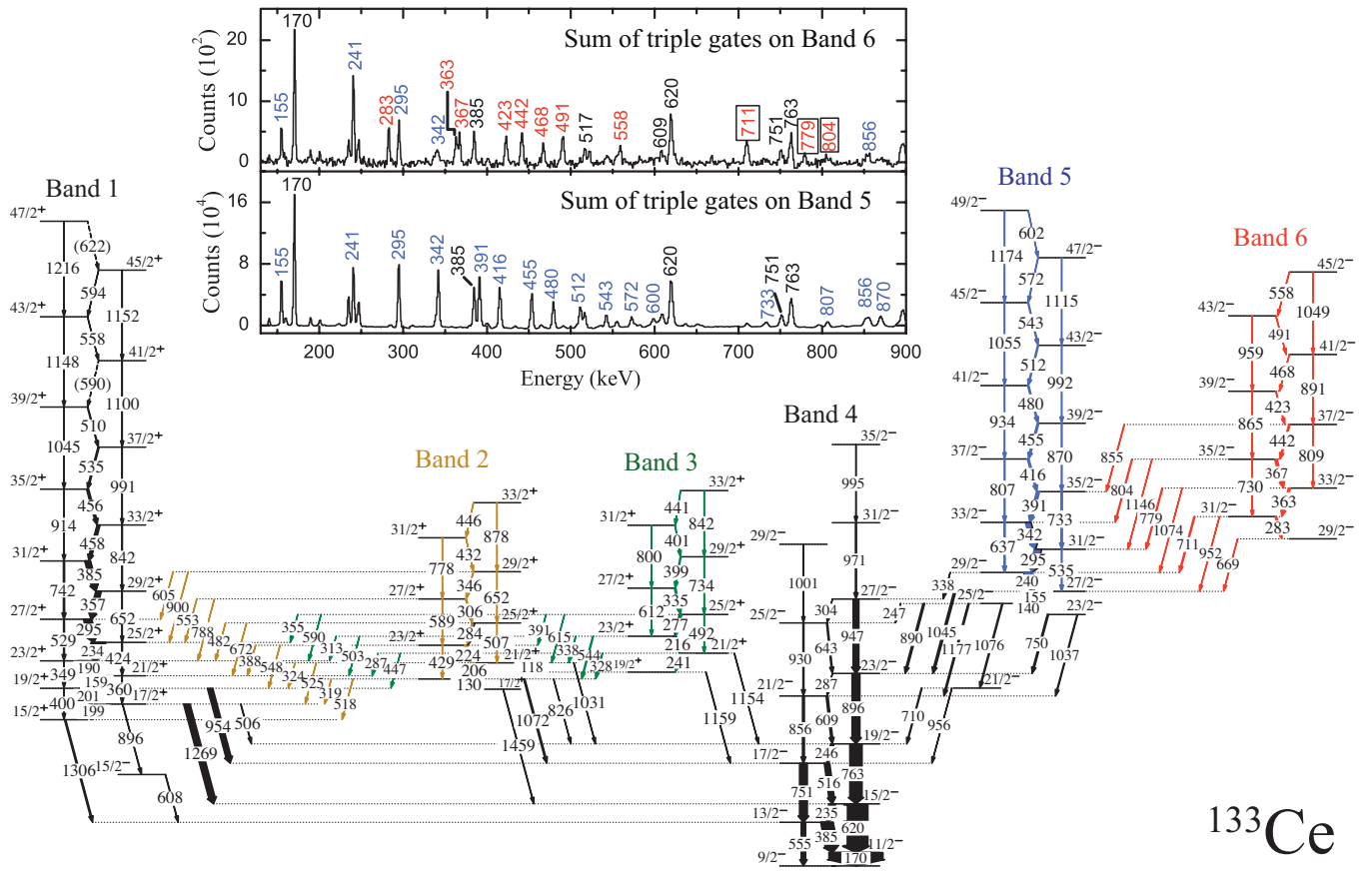
FIG. 1: (Color online) Partial level scheme of ^{133}\text{Ce} showing the previously-known bands and the partner bands identified in this work. All transitions within and out of a band are shown in the same color. The lowest level shown ( I^\pi = \frac{9}{2}^- ) is not the ground state, but an isomer with an excitation energy of 37.2 keV [31]. Inset: Background-subtracted \gamma - \gamma - \gamma coincidence spectra from different gate combinations between Bands 5 and 6. Black-, blue-, and red (with arrows)-colored transitions represent members of Bands 4, 5, and 6, respectively. The interconnecting transitions between Bands 5 and 6 are identified by boxes around the transition energies.
