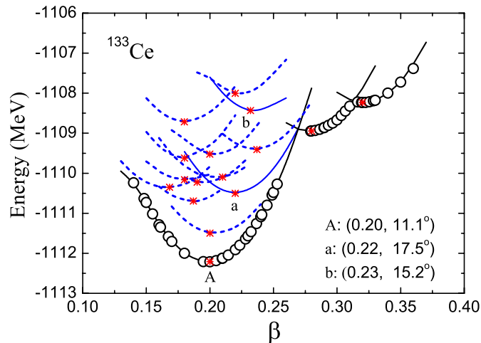
FIG. 3: (Color online) Potential-energy curves in adiabatic (open circles) and various configuration-fixed \beta -constrained (solid and dashed curves) RMF calculations with the parameters set PK1 [42] for ^{133}\text{Ce} . The energy minima are represented as stars. The letters A, a, and b denote the calculated ground state, Band 2, and Band 5, respectively.
