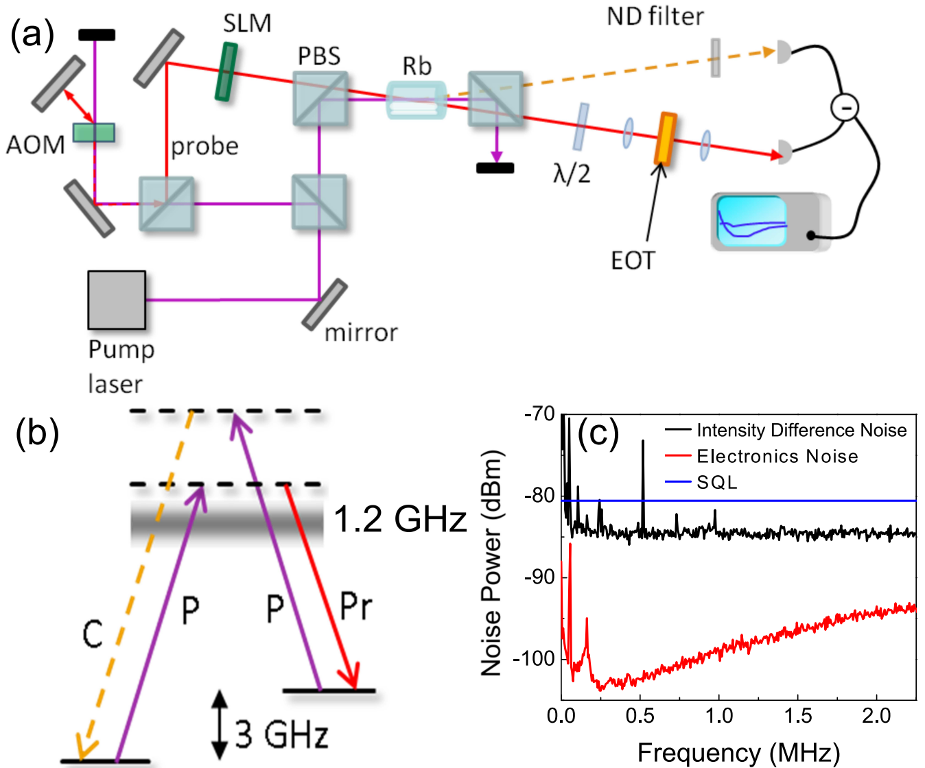
FIG. 1. (Color online) (a) A schematic of the 4WM experiment with abbreviations SLM: spatial light modulator, PBS: polarizing beam splitter, AOM: acousto-optic modulator, and ND: neutral density. (b) The energy level diagram for the D1 line in Rb at 795 nm, showing two pump (P) photons absorbed by the vapor and two subsequent probe (Pr) and conjugate (C) photons re-emitted with quantum correlations. (c) A typical squeezing spectrum showing a maximum of 4 dB of squeezing at frequencies above 1 MHz. This squeezing spectrum was acquired with 10% attenuation on the probe and conjugate corresponding to the transmission through an indium tin oxide coated glass substrate.
