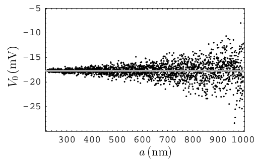
FIG. 1: The residual potential difference between a Ni-coated sphere and a Ni-coated plate as a function of separation. The mean value of V_0 is shown by the gray line.
