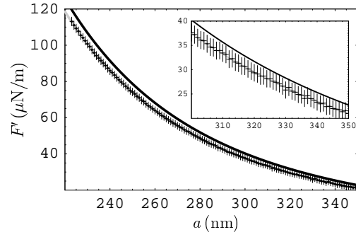
FIG. 4: Comparison between the experimental data for F' plotted at a 95% confidence level and theory (black and gray bands computed using the Drude and plasma model approaches, respectively).
