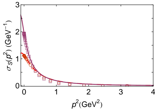
FIG. 1. \sigma_S(p^2) in Eq. (4a) – RL kernel: solution (open circles) and interpolation function (long-dashed curve); and DB kernel: solution (open squares) and interpolation function (solid curve). In the chiral limit at large p^2 , \sigma_S(p^2) \sim 1/p^4 .
