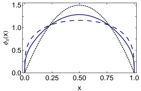
FIG. 2. Computed distribution amplitude at \zeta = 2 \text{ GeV} . Curves: solid, DCSB-improved kernel (DB); dashed, rainbow-ladder (RL); and dotted, asymptotic distribution.
