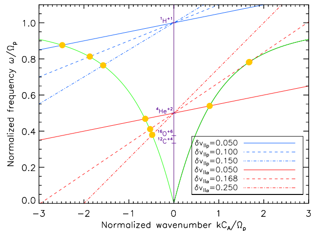
FIG. 1. The dispersion relation for parallel propagating ion-cyclotron waves (green curve) and the resonance criteria given in equation Eqn. (2) for \text{H}^+ (blue) and \text{He}^{2+} (red) streaming along \mathbf{B} at different \delta v_{\parallel i} . Gold circles indicate wave resonances.
