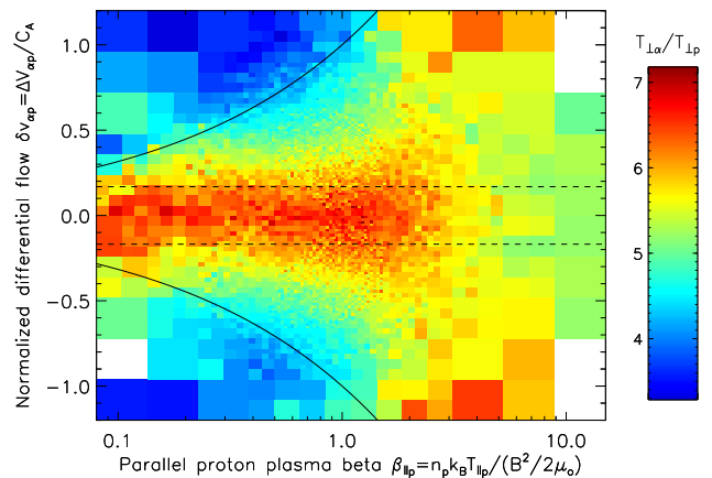
FIG. 2. T_{\perp\alpha} / T_{\perp p} in the \beta_{\parallel p} - \delta v_{\alpha p} plane. Dashed lines indicate \pm \delta v_{\alpha p}^c , the speed below which the core of the He^{2+} VDF should experience multiple resonance. Solid lines indicate \pm \delta v_{\alpha p}^t , the speed beyond which only the tail of the He^{2+} is heated.
