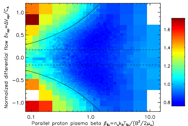
FIG. 3. H^+ temperature anisotropy T_{\perp p} / T_{\parallel p} in the \beta_{\parallel p} - \delta v_{\alpha p} plane. Threshold conditions are the same as in Fig. 2. When |\delta v_{\alpha p}| > \delta v_{\alpha p}^c and the He^{2+} become non-resonant, the H^+ take on a large anisotropy consistent with cyclotron resonance.
