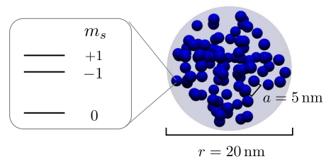
FIG. 1: High-density NV spin ensemble distributed randomly within a sphere of diameter r , with an average distance a . The NV centers have three internal spin states that are split by a zero-field splitting and a Zeeman field.
