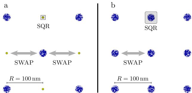
FIG. 4: Scalable architectures with collectively enhanced interactions, corresponding to a lattice spacing of R = 100 nm, compatible with sub-wavelength optical addressing. (a) Individually addressable NV qubits (yellow) are used for single qubit operations (SQR), whereas the collectively enhanced interaction with an ensemble is used to mediate two-qubit gates via SWAP operations. (b) NV ensembles are used as collective qubits, where also single qubit operations are performed using the collective |W\rangle state.
