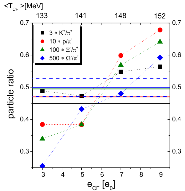
FIG. 2. (Color online) Hadron ratios as a function of the transition energy density for central Pb+Pb reactions at \sqrt{s} = 2.75 TeV. The symbols denote the calculations, the line depict the experimental data.
