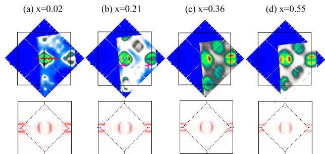
FIG. 3: (color online) Comparison of the Fermi surface at k_z = \pi plane between the ARPES results [15] (top panel) and our results (bottom panel) in 1-Fe zone for different Ru concentration x = 0.02 (a), 0.21 (b), 0.36 (c) and 0.55 (d). The dashed lines marks the true 2-Fe Brillouin zone boundaries.
