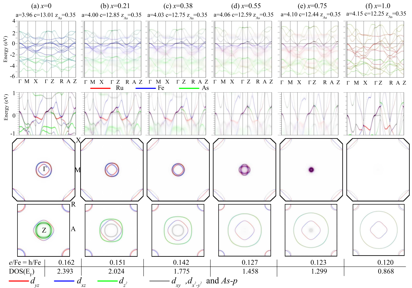
FIG. 1: (color online) The lattice constants (Å) [13, 24, 25], band structure (the first panel), low energy band structure (the second panel), the Fermi surface around \Gamma point with k_z = 0 (the third panel) and around Z point with k_z = \pi (the last panel) for \text{Ba}(\text{Fe}_{1-x}\text{Ru}_x)_2\text{As}_2 with different Ru concentration x = 0 (a), 0.21 (b), 0.38 (c), 0.55 (d), 0.75 (e) and 1.0 (f). Orbital characters of Fe, Ru, and As are distinguished by color given in the legend. Resulting carrier density per Fe, and density of states at the Fermi level N(E_F) per (eV Fe) are given below the plots.
