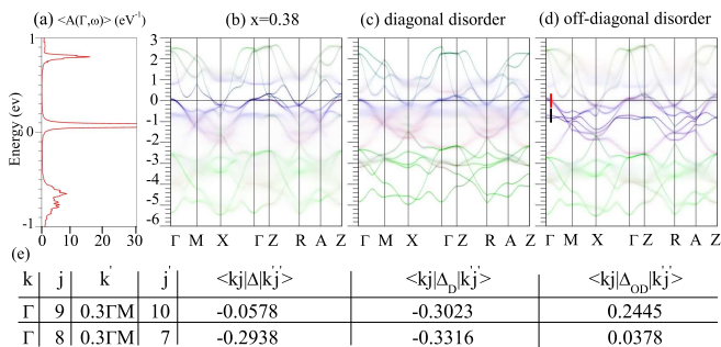
FIG. 2: (color online) Spectral function (a) and band structure for system with two types of disorder (b), with only the diagonal disorder (c), and with only the off-diagonal disorder (d) for disordered \text{Ba}(\text{Fe}_{0.62}\text{Ru}_{0.38})_2\text{As}_2 . (e) single-impurity induced coupling between the Bloch orbitals near and far from the chemical potential, indicated by the black and red segments in (d).
