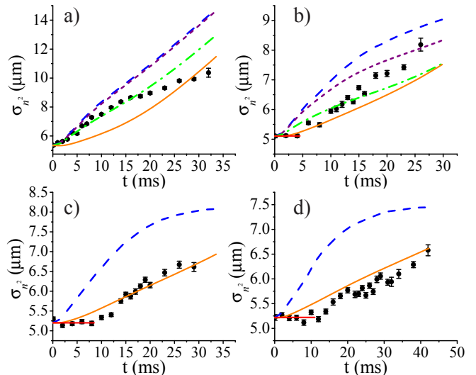
FIG. 2: (Color online) Transverse RMS widths of the directly measured density squared distributions as a function of time for (a) V_0 = 7.25 E_R , (b) 9.25 E_R , (c) 11 E_R , (d) 13 E_R . Each data point is the average of 10 measurements. The error bars represent our random uncertainty and are the quadrature sum of the statistical noise and the uncertainty from the density dependence of the absorption beam lensing. There is an overall, systematic uncertainty of 0.5 \mu\text{m} associated with the imaging resolution; comparable shifts of the initial size simply shift the theoretical curves at early times (below 10 ms), followed by a gradual divergence of the curves at longer times. The blue dashed line is the result of a mean-field calculation of the dynamics with no random phase between the tubes ( \eta = 0 ). The purple dotted line is for \eta = 0.2 , the green dash-dotted lines are for \eta = 0.4 (a) and \eta = 0.5 (b), and the orange solid line is for \eta = 1 . The red horizontal line is the mean of the t < t_c data.
