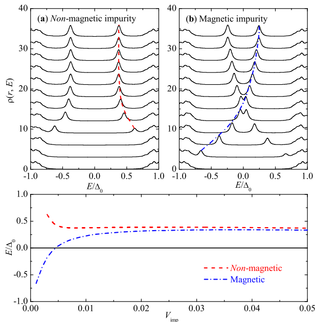
FIG. 1: (color online) Bound states induced by a non-magnetic delta-like impurity (a) and by a magnetic delta-like impurity (b), V_{\text{imp}}^\sigma(\mathbf{r}) = V_{\text{imp}}^\sigma \delta(r) , in a topological superfluid at \hbar = 0.7E_F , as shown by the peaks in the total local density of state (LDOS) \rho(r, E) at k_F r = 2 . Here, \rho(r, E) = \sum_\sigma \rho_\sigma(\mathbf{r}, E) and \rho_\sigma(\mathbf{r}, E) = (1/2) \sum_\eta [|u_{\sigma\eta}|^2 \delta(E - E_\eta) + |v_{\sigma\eta}|^2 \delta(E + E_\eta)] . The dashed and dash-dotted lines highlight the resonance peak position and the energy of bound states. From bottom to top, the impurity strength increases from V_{\text{imp}} = 0 to V_{\text{imp}} = 0.011r_F^2 E_F , in steps of 0.001r_F^2 E_F . The curves are offset for clarity, except for the lowest curve at V_{\text{imp}} = 0 . (c) The energy of bound states as a function of the impurity strength, in units of the gap parameter at the trap center in the absence of impurity, \Delta_0 \simeq 0.307E_F .
