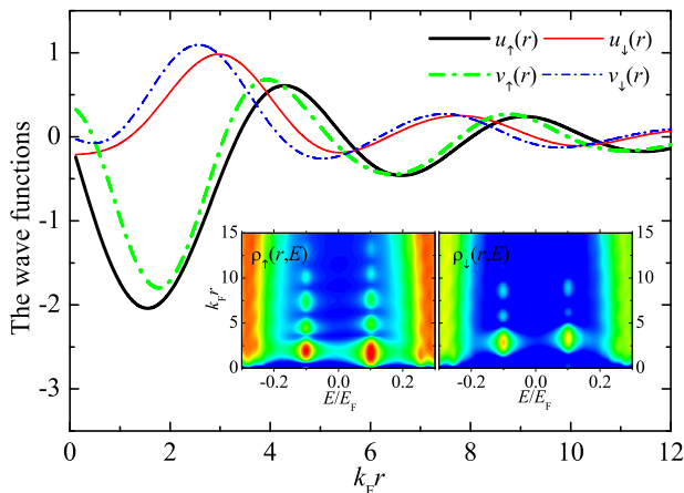
FIG. 3: (color online) The wave-function of the universal bound state, induced by either non-magnetic or magnetic impurity in the strong scattering limit. The inset shows the linear contour of LDOS for spin-up and spin-down atoms near the impurity site.
