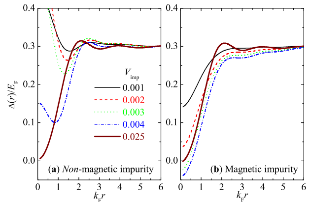
FIG. 2: (color online) Gap parameter as a function of impurity strength V_{\text{imp}} (in units of r_F^2 E_F ), for a non-magnetic impurity (a) and for a magnetic impurity. In the limit of strong impurity scattering, the gap parameter has the same spatial distribution, no matter the impurity is non-magnetic or magnetic.
