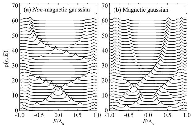
FIG. 4: Loss of the universal bound state for an extended impurity. Here, we take a gaussian-shape scattering potential, V_{\text{imp}}^\sigma(\mathbf{r}) = [V_{\text{imp}}^\sigma/(\pi d^2)] \exp[-r^2/d^2] , with width k_F d = 0.5 . From bottom to top, the impurity strength increases from V_{\text{imp}} = 0 to V_{\text{imp}} = 0.06r_F^2 E_F , in steps of 0.002r_F^2 E_F . Other parameters are the same as in Fig. 1.
