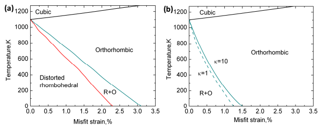
FIG. 1. (color online) Strain-temperature phase diagrams of \text{BiFeO}_3 thin film from phase-field simulations. (a) Under short-circuit boundary condition and (b) under open-circuit boundary conditions.
