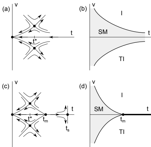
FIG. 2: (a,c) RG flow diagrams based on (12). The stable fixed point at (t, v) = (0, 0) is the symplectic metal (SM). The unstable fixed points at (t^*, \pm v^*) approach the KT transition for \epsilon = 1 - N \ll 1 and for N \rightarrow 0 are identified with the Anderson transition. (c) includes a third fixed point at (t_m, 0) , along with a fixed point at (t_s, 0) describing a direct transition between TI and I. (b) and (d) are phase diagrams corresponding to (a) and (c).
