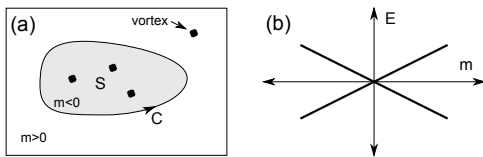
FIG. 1: (a) A 2D TI ( m < 0 ) in region S with boundary C is surrounded by trivial insulator ( m > 0 ). The sign of Z_{\text{eff}} depends on the number of vortices in S . (b) For m = 0 the eigenvalues of \mathcal{H}^{\text{eff}} in (10) exhibit a linear zero crossing, which leads to a vanishing vortex fugacity.
