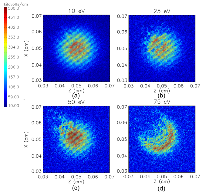
FIG. 4. Electric field magnitude at t = 50 \text{ ps} for 3 \times 10^{12} \text{ W}/\text{cm}^2 laser intensity, \theta = 90^\circ , and varying T_0 : (a) 10 eV ( F = 11 ), (b) 25 eV ( F = 3.8 ), (c) 50 eV ( F = 2.7 ), and (d) 75 eV ( F = 2.2 ).
