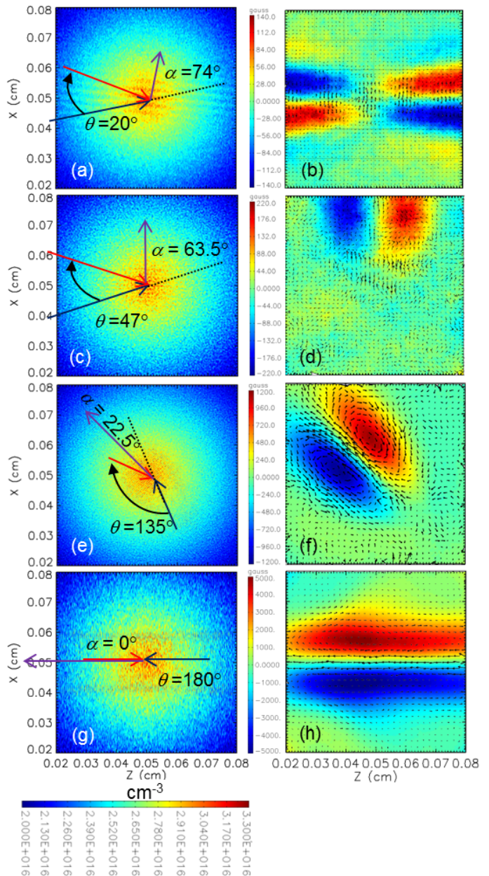
FIG. 2. Beat wave modulated electron density contours (left column) at t = 20 ps for (a) 20^\circ , (c) 47^\circ , (e) 135^\circ , and (g) 180^\circ ; magnetic field contours and electron mean velocity vectors (right column) for (b) 20^\circ at 50 ps, (d) 47^\circ at 50 ps, (f) 135^\circ at 100 ps, and (h) 180^\circ at 100 ps. This is for laser intensities of 3 \times 10^{12} W/cm ^2 and 50-eV plasma.
