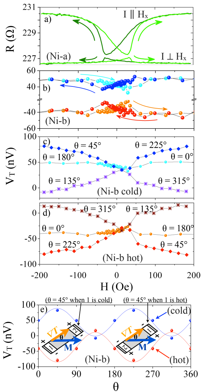
FIG. 4. (color online). a) AMR data for Ni-a. b) V_T versus H for one detector on Ni-b when hot and cold for up and down H sweeps. c) V_T versus H for Ni-b when cold for one sweep direction at various \theta (the angle between M and \nabla T and d) when hot. e) V_T vs \theta for Ni-b when the detector is hot and cold with \sin\theta\cos\theta fit. Data when hot appear reversed due to the sign change introduced by reversing \nabla T . Insets: Schematics show the sign change for V_T when \nabla T is reversed.
