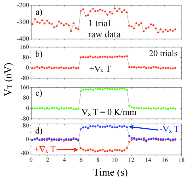
FIG. 2. (a) Example raw data for V_T across a Pt detector. (b) Averaged data when hot ( \nabla_x T = 62.5 \text{ K/mm} , and (c) when both sides of the film generated equally leaving only the background thermovoltage generated by \nabla T_y . (d) Hot and cold measurements ( \nabla_x = \pm 62.5 \text{ K/mm} ) after subtracting the \nabla T_y contribution. For all measurements, the heater is cycled on at 6 seconds and off at 11 seconds.
