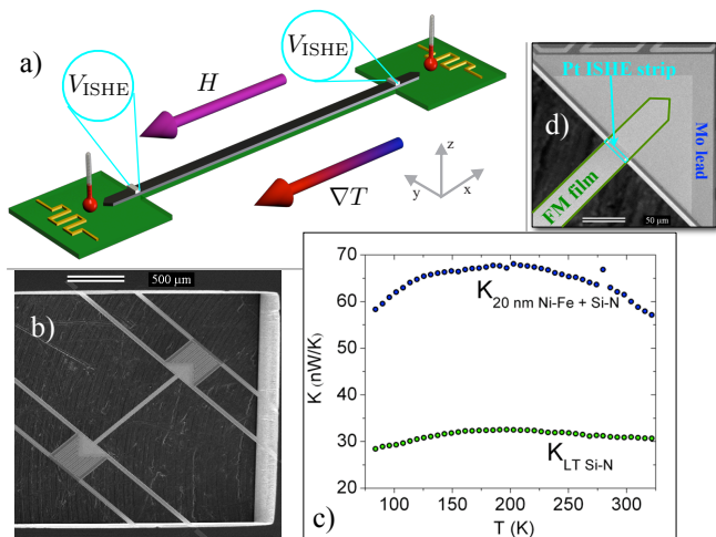
FIG. 1. (a) Schematic of the thermal isolation platform with \nabla T and H applied in the negative x -direction, (b) SEM micrograph of the platform, and (c) plot of thermal conductance vs T for a Si-N bridge and a 20 nm Ni-Fe film deposited on a Si-N bridge. (d) SEM micrograph of one island shows a triangle-shaped lead for measuring film resistance and thermopower, false color outlines show a 20 nm thick Ni-Fe film and a 10 nm thick Pt spin detector.
