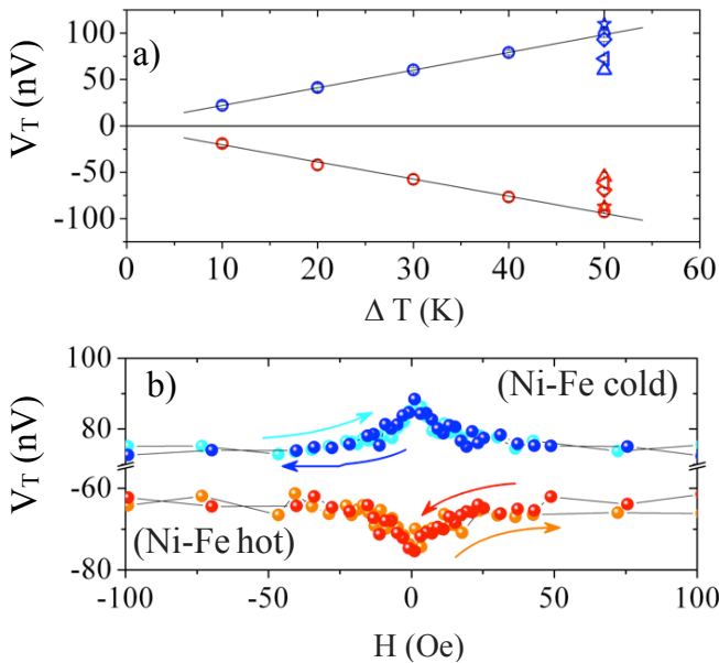
FIG. 3. (color online). V_T versus \Delta T for Ni-Fe ( H = 100 Oe, \theta = 0 ). a) V_T for one detector when hot and cold with a linear fit. Additional points at \Delta T = 50 K are for the same detector on four additional Ni-Fe films. The same trends occur for the other Pt detector (not shown). b) V_T versus H (applied in the \pm \hat{x} direction) for one detector on a Ni-Fe film when hot and cold for up and down H sweeps.
