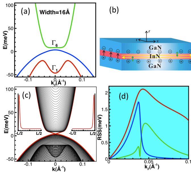
FIG. 3: (color online) (a) Band structure of a 16 Å GaN/InN/GaN QW obtained from the six-band effective Hamiltonian. (b) Schematic of a infinite long spin Hall bar with a width (along y ) of 1000 Å. The thickness along the [0001] growth direction (labeled as z ) comprises the InN QW plus two 200-Å-thick GaN barrier layers on either side. The yellow lines show the helical edge states, and the green arrows show the spin orientation. The short black arrows indicate the polarization-induced electric field. (c) Band structure of the Hall bar obtained by solving the effective six-band model. The insets show the density distributions of one Kramers pair of edge states: on the left the spin-up state at k_{\parallel} = -0.1 \text{ \AA}^{-1} , on the right the spin-down state at k_{\parallel} = 0.1 \text{ \AA}^{-1} . (d) Rashba spin splitting of electron (green), HH (blue) and LH (red) subbands.
