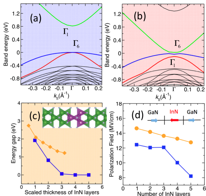
FIG. 2: (color online) (a) and (b) Band structure of a GaN/InN/GaN QW around the \Gamma point for 2 and 4 ML of InN, based on first-principles DFT-HSE calculations. The green lines represent electron states, red lines light-hole states, and blue lines heavy-hole states. (c) Calculated energy gaps as a function of the thickness of InN layers for polar ([0001]) (blue squares) and non-polar ([10 \bar{1} 0]) (orange diamonds) GaN/InN/GaN QWs. The thicknesses were scaled to the thickness of 1 ML of InN in a polar QW and therefore correspond to the number of InN layers in the polar case. The inset shows a [10 \bar{1} 0] QW with two InN layers. (d) Polarization field as a function of number of inserted InN layers calculated by DFT-HSE (blue squares) and based on theoretical polarization constants (orange circles). The blue and red block arrows in the inset show the polarization direction of GaN and InN regions [19].
