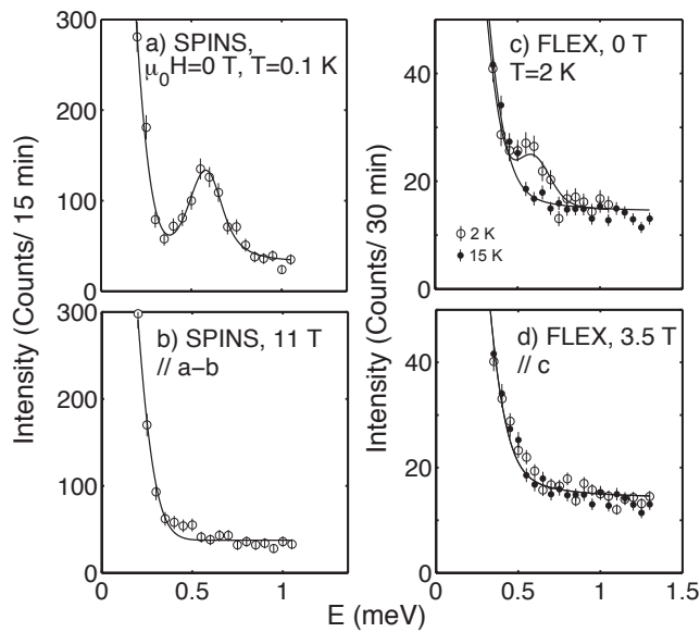
FIG. 1. Panel a ) and b ) illustrate the \mathbf{Q}=(1/2,1/2,1/2) resonance in zero field ( T=0.1 K) and 11 T (near H_{c2} ) along the [1\bar{1}0] direction. Panels c – d ) are acquired with the field applied along the c axis. The curves are fits to a simple harmonic oscillator and a background originating from incoherent elastic scattering. The temperature independent peak at E=0 meV results from background associated with strong nuclear incoherent scattering and is not magnetic in origin.
