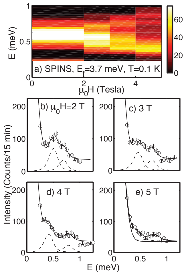
FIG. 3. (color online) The magnetic field dependence of the resonance peak at 0.1 K taken on SPINS. a ) background corrected intensity as a function of magnetic field. b ) - e ) The solid lines are fits to two damped harmonic oscillators and the dashed lines indicate the individual fits. An overall background fixed to the 11 T scan was also subtracted and is represented by the solid line in e ) for the 5 T data.
