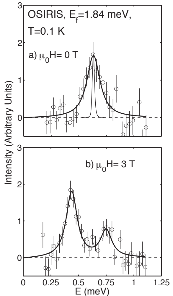
FIG. 2. a ) illustrates a high resolution scan through the spin resonance at zero applied field. The solid curve centered at 0.6 meV illustrates the resolution function on OSIRIS with a full width of 0.025 meV. The resolution is derived from the elastic line and it was assumed not to change significantly between 0 and 0.5 meV (Ref. 25). b ) demonstrates the splitting of the resonance into two peaks under an applied field of 3 T. A 10 K background was subtracted from the scans.
